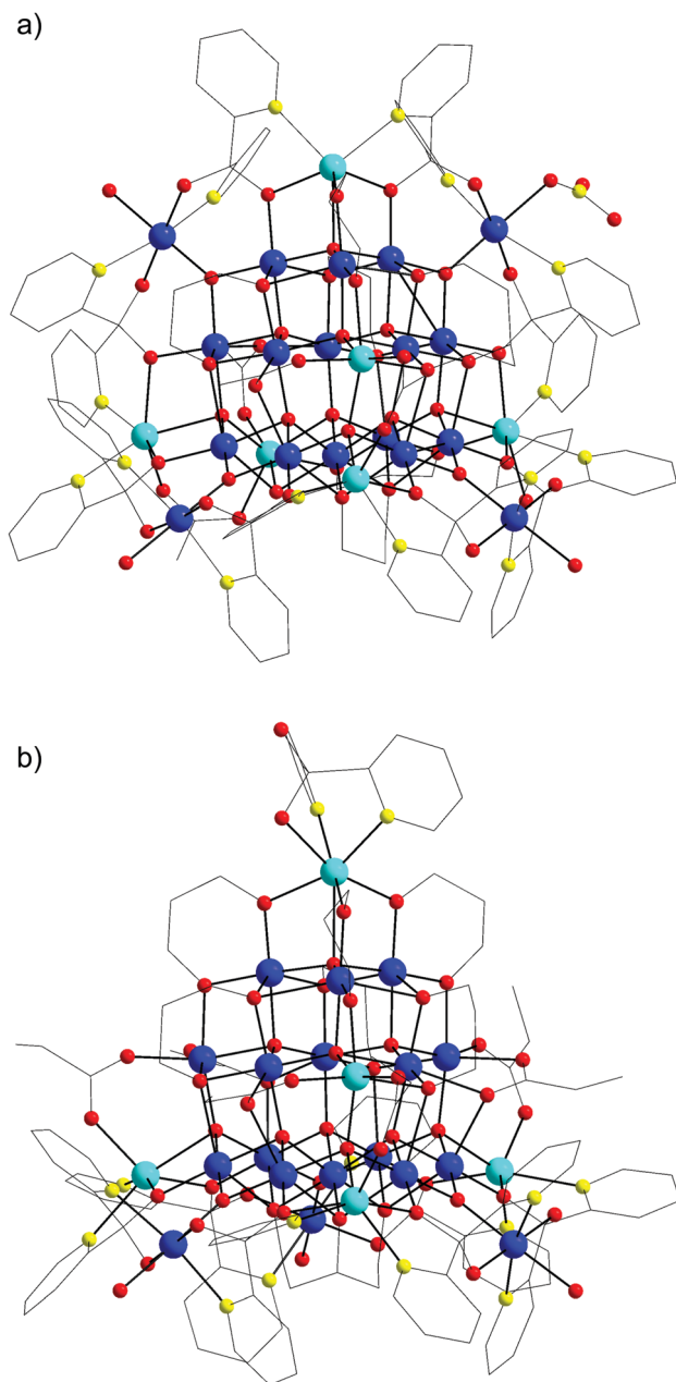
Fig. 1 Representations of the molecular structures of compounds (a) 1 and (b) 3 . Colour code: Mn II , turquoise; Mn III , blue; O, red; N, yellow; C, grey. H atoms and the counter ions are omitted for clarity.
