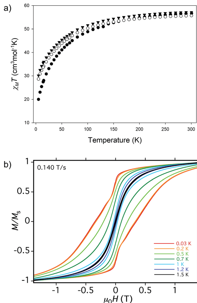
Fig. 3 (a) \chi_M T versus T plots for complexes 1 ·22 \text{H}_2\text{O} (▼), 2 ·33 \text{H}_2\text{O} (○) and 3 ·28 \text{H}_2\text{O} (●) at 0.1 T and (b) magnetization ( M ) versus applied magnetic field ( \mu_0 H ) hysteresis loops for a single crystal of 1 ·2.5 \text{H}_2\text{O} ·solvent at the indicated temperatures and a fixed field sweep rate of 0.140 T \text{s}^{-1} . The magnetization is normalized to its saturation value, M_s .
