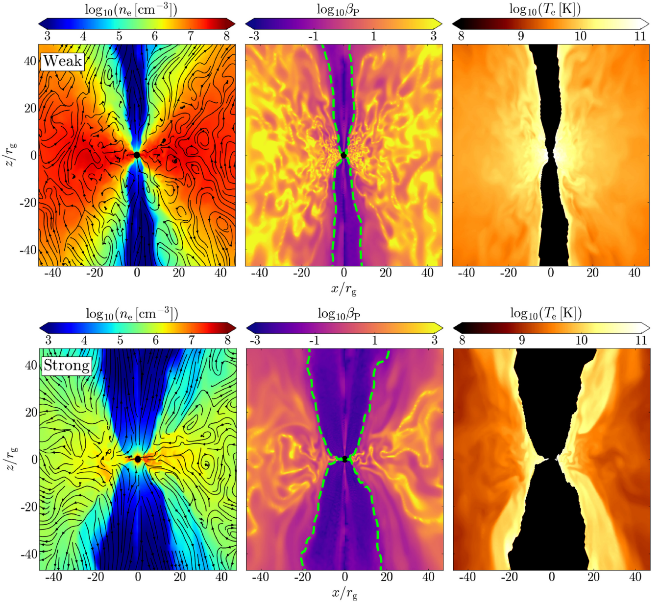
Figure 2. Strongly magnetized discs lead to wider jets, magnetically dominated winds and lower disc densities and temperatures as compared to their weak disc counterparts. We show x-z cross-sections of the electron number density n_e (with velocity streamlines in black), plasma- \beta and electron temperature T_e from our GRMHD simulations: (top row) weak-field disc model Weak and (bottom row) strong-field disc model Strong , scaled to Sgr A* according to Table 1. We also indicate the jet boundary (approximated as magnetization \sigma_M = 1 ) in green for the plasma- \beta plots. Further, the jet is cut out (black region) in the T_e plots, since we do not account for the jet spine emission in our radiative scheme. Snapshots are taken at approximately 28,000 r_g/c .
