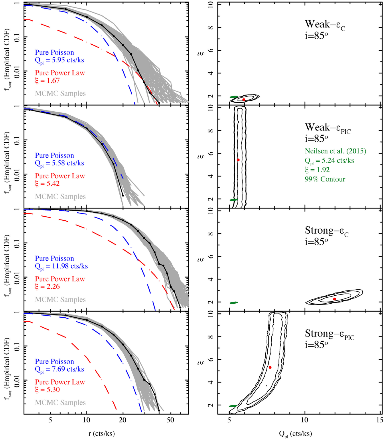
Figure 12. We show cumulative distribution functions ( f_{\geq r} ) as a function of the flux count rate ( r ) for the X-ray 2–8 keV light curve constructed from the four different radiative models with inclination angle 85^\circ . The radiative model CDF (black line) is fitted with a Poissonian component (blue-dashed) to represent the quiescent flux distribution and a variable process in the form of a power-law (red-dashed), as indicated by the best-fitting values of the Poisson rate Q_{\text{pl}} and the power-law index \xi (see Section 5.3). In order to directly compare to Sgr A* X-ray CDFs from Neilsen et al. (2015), we add a quiescent background count rate to the flux distribution. The grey lines in left-hand panels are the results of MCMC simulations from the joint probability distribution of Q_{\text{pl}} and \xi . We also show probability contour plots in the right panels that illustrate the correlation between parameters Q_{\text{pl}} and \xi (panels b and d), with contours corresponding to 68 per cent, 90 per cent, and 95 per cent confidence levels. The green oval indicates the Neilsen et al. (2015) best fit with the 99 per cent confidence contour. The Weak- \epsilon_C parameters fits perform relatively better than the other models when comparing to the Sgr A* best-fitting values. All other models either do not show a significant power-law component or have very high Q_{\text{pl}} .
