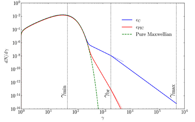
Figure 1. The electron distribution function for a cell in the magnetized inner accretion flow for both types of non-thermal models considered: constant power-law \epsilon_C and varying power-law \epsilon_{\text{PIC}} . We assume an electron temperature T_e = 10^{11} K, magnetization \sigma_M = 0.5 , R_{\text{low}} = 10 , R_{\text{high}} = 40 , magnetic field B = 40 G, here located at a radius of 5 r_g from the BH. For the power-law distributions, we show the minimum and maximum electron Lorentz factors and the break Lorentz factor. The dotted blue and red lines illustrates the break in the power law due to synchrotron cooling. For comparison, we also show the relativistic Maxwell-Jüttner distribution for these parameters.
