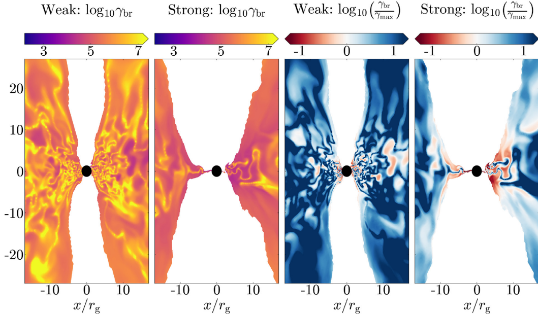
Figure 4. 2D cross-sections of the break Lorentz factor \gamma_{br} as determined from equation (3.2) and the ratio of \gamma_{br} and the power-law distribution Lorentz factor cutoff \gamma_{max} . Most of the synchrotron cooling occurs within 5–10 r_g of the BH, where \gamma_{br} < \gamma_{max} . We take the same snapshots for this figure as the ones shown in Fig. 3. As in Fig. 3, here we exclude the jet funnel from our calculations.
