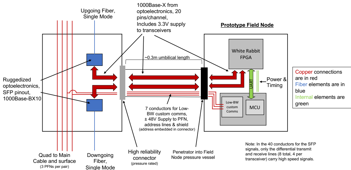
Figure 2: Block diagram of the High Speed Copper breakout and Prototype Field Node design for the Fiber Test System. In contrast with the full-array version shown in Figure 1 panel A, the prototype does not include connections to DOMs but includes a separate controller board for communications with the surface over long-run copper. In the non-prototype Field Node, microcontroller (MCU) functions will be handled on the Zynq chip also housing the White Rabbit functionality.
