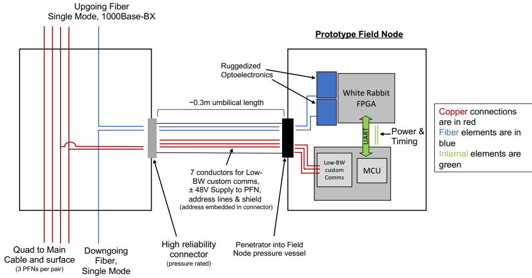
Figure 3: Block diagram of the Hybrid Fiber Penetrator breakout and Prototype Field Node design for the Fiber Test System. In this design, fibers running to the Prototype Field Node simplify optoelectronic conversion but add the risk of connector flooding, and the complexity of making fiber optic connections in South Pole conditions.
