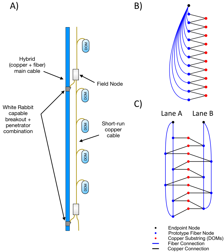
Figure 1: A) Diagram of the overall IceCube-Gen2 Fiber Communications option pointing out main features of the system. B) the "classic" fiber topology, with a single fiber going to each Field Node. C) the interspersed fiber topology, using fewer fibers and achieving greater redundancy than the "classic" topology by dividing connections into two redundant lanes. We also minimize the fiber length between adjacent nodes along each lane, thereby maximizing signal regeneration.
