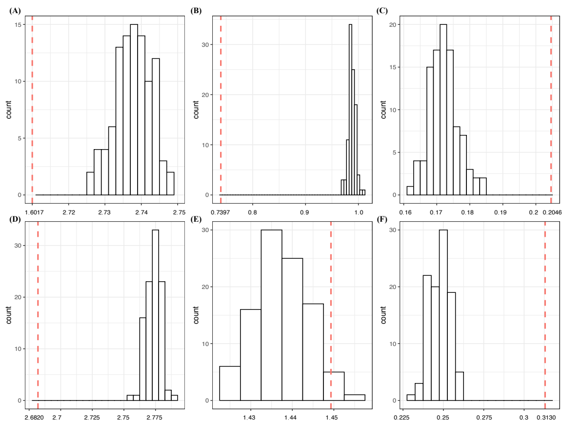
Figure 6. Determine when to stop CEDA-based selection for major factors: (A) ( aX, aZ^* ); (B) ( aX, aZ, vY0^* ); (C) ( aX, aZ, vX0, vY0^* ) on Y = (pfX_X, pfX_Z) ; (D) ( spinD, aY^* ); (E) ( spinD, vZ0, aY^* ); (F) ( startSp, x0, vZ0, vX0^* ) on Y = (ax, az) . Each red dotted line indicates the conditional entropy given the feature set, and the histogram is the conditional entropies of samples generated with the *-marked feature being replaced by a random noise feature.
