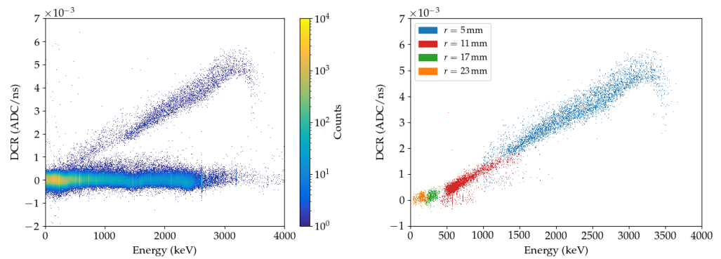
(a) DCR vs. energy ( r = 5 mm).
