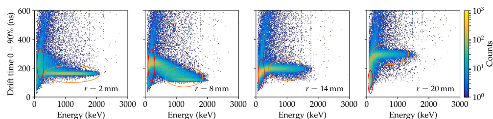
Figure 15. Correlations between the drift time (0–90%) and E_{\beta}^{\text{obs}} at selected r . The red vertical and orange horizontal ellipses in the distributions indicate two event populations.
