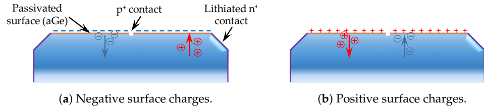
Figure 3. Effect of (a) negative and (b) positive charges on the passivated surface of a PPC germanium detector. In the case of negative (positive) surface charges, holes (electrons) are attracted to the surface, whereas electrons (holes) are repelled.
