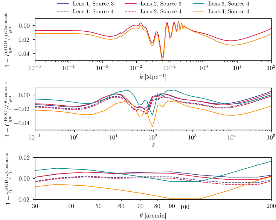
Figure A1. COSMOSIS code comparison residuals for C_{gm}(\ell) and \gamma_t(\theta) for 6 bins of interest. The bias values per each of the four lens bins [1,2,3,4] are \bar{b}_g = [1.2, 1.6, 1.7, 1.7] , respectively. For the first panel, we have used the mean redshift of each lens redshift bin to calculate and compare the galaxy-matter cross power spectra. The other two panels show the projected power spectrum and tangential shear comparison for the average over the redshift distributions. These comparisons are done using the following parameters for a flat \Lambda CMD cosmology: \Omega_m = 0.25 , \Omega_b = 0.044 , \sigma_8 = 0.8 , n_s = 0.95 , H_0 = 70 \text{ km s}^{-1} \text{ Mpc}^{-1} and \Omega_v = 0 . Furthermore, note that the redshift distributions, n(z) , are not the same as what we used throughout this paper, but both our and the COSMOSIS results used the same n(z) for lenses and sources.
