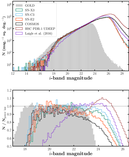
Figure 13. Upper: Raw number counts (uncorrected for incompleteness) in the i -band for our four Deep Fields (COADD.TRUTH depth level), together with the main DES survey, HSC PDR-1 UltraDeep (COSMOS + SXDS) and the Laigle et al. (2016) UltraVISTA/COSMOS catalogue. The fall off in number counts at the bright end with respect to the GOLD sample is largely due to masking of bright stars and saturation (for the Laigle et al. 2016 catalogue). Lower: Ratio of number counts to a fiducial power-law distribution.
