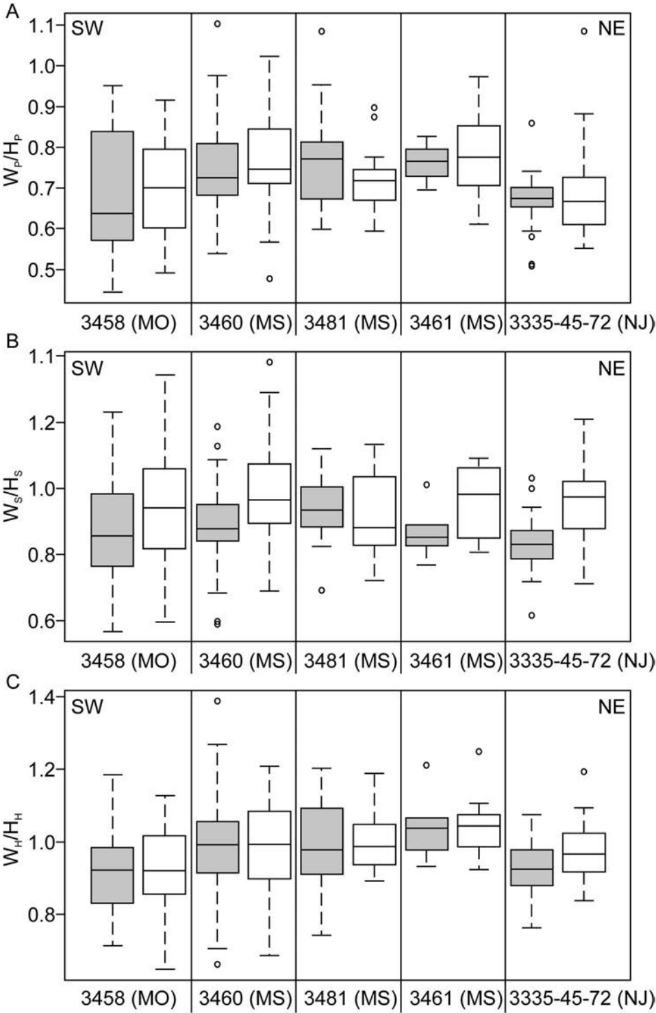
FIGURE 5. Box-and-whisker plots showing whorl compression ratios of Discoscaphites iris specimens plotted geographically from SW (Missouri) to NE (New Jersey). A, W_p/H_p , B, W_s/H_s , C, W_h/H_h . Box edges represent the first and third quartile, horizontal black line is the median. Whiskers illustrate the minimum and maximum. Circles are outliers. Data are presented separately for each dimorphy; gray shaded boxes are macroconchs, white boxes are microconchs. Compression ratios were not measured on specimens from Brazos River, Texas.
