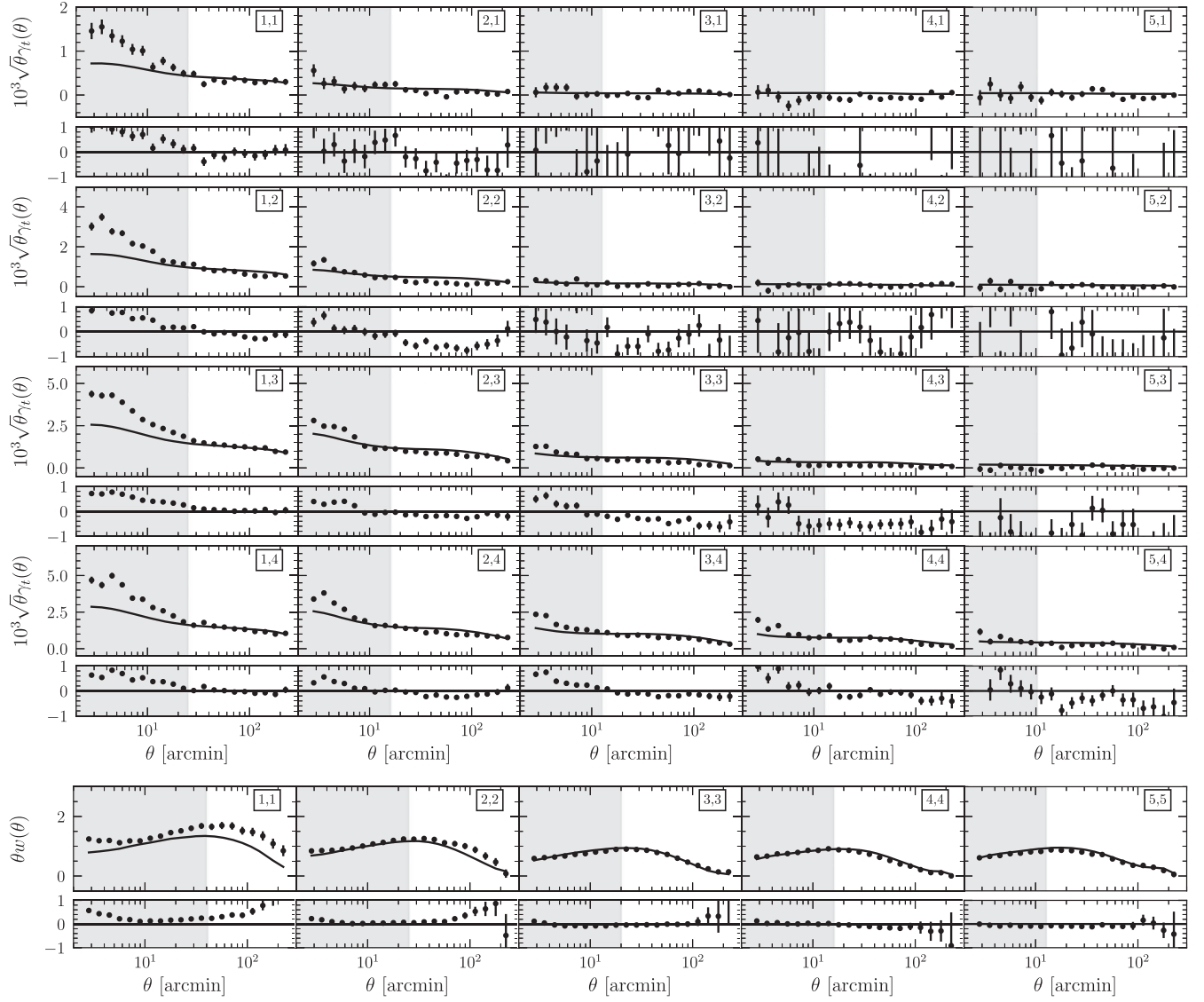
FIG. 3. Comparison of \gamma_t(\theta) and w(\theta) between BUZZARD (lines) and the measurements from the Y3 data using the REDMAGIC lens sample (points), with error bars given by the fiducial Y3 covariance matrix. Shaded regions indicate the angular scale cuts applied in the fiducial 3 \times 2 -point analysis. Rows alternate between showing the measured signals and the fractional difference between data and simulations. Numbers in each panel label the bin combinations shown, with the numbers in the \gamma_t(\theta) panels representing the lens-source bin pair and numbers in w(\theta) panels denoting the lens bins alone. The intent of this comparison is to gauge how well the galaxy clustering and lensing properties in BUZZARD match those observed in the data, with the caveat that disagreement may arise due to differences in cosmology, and source and lens galaxy redshift distributions. Agreement in w(\theta) is generally better than for \gamma_t(\theta) especially for the second through fifth lens bins, which may be a result of slightly different source redshift distributions between the simulations and data, especially where there is significant overlap between source and lens redshift distributions. We also observe a marked deficit of power on small scales in \gamma_t(\theta) for the first lens bin at smaller scales than those used in the analysis, part of which is likely due to resolution effects in BUZZARD. The excellent match between \gamma_t(\theta) on larger scales in the first lens bin is interesting in light of the large discrepancy in the amplitude of w(\theta) between the DES Y3 data and BUZZARD for this lens bin. The DES Collaboration [44] demonstrates that under the assumption of LCDM the REDMAGIC w(\theta) and \gamma_t(\theta) imply bias values that differ by 12%, so this may play some role in the discrepancies seen between the BUZZARD and DES Y3 w(\theta) measurements in the first lens bin.
