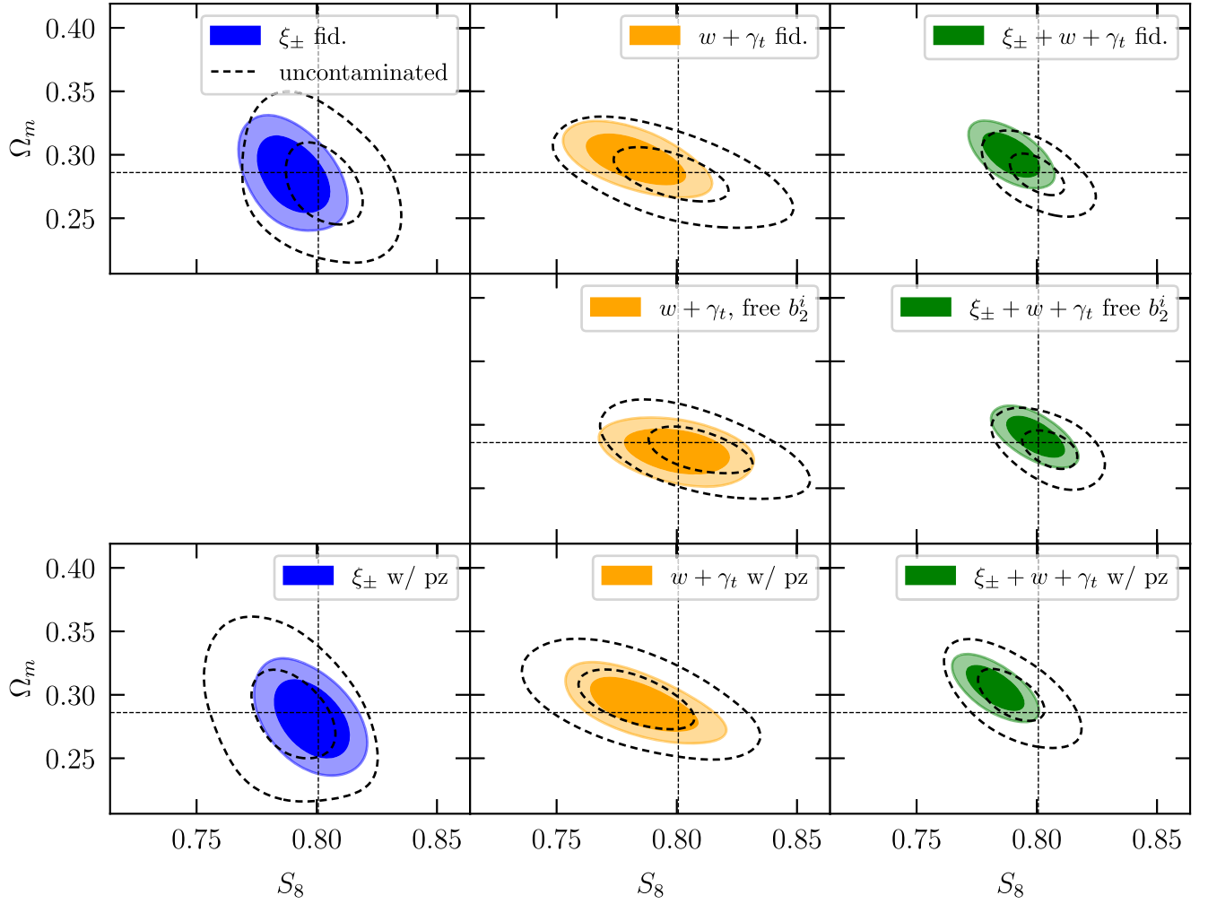
FIG. 8. Constraints on S_8 and \Omega_m from 1 \times 2 - (left), 2 \times 2 - (middle), and 3 \times 2 -point (right) analyses on the mean data vector from the full suite of simulations. Top: constraints marginalizing over only cosmology, linear bias, and IAs, assuming the true source and lens redshift distributions. Posteriors obtained using the mean BUZZARD data vector are shown as solid lines, while dashed contours use a data vector generated at the true cosmology of the simulations with the best-fit linear bias model from analysis configuration A1, i.e., the blue line in Fig. 7. The shaded BUZZARD contours are the 1/\sqrt{18} and 2/\sqrt{18} confidence regions, while the dashed contours represent the 0.3 and 1\sigma confidence regions for a single simulation realization. The crosshairs represent the true BUZZARD cosmology, and the difference between the dashed contours and these is a product of parameter projection effects. Middle: same as the top row, but posteriors are obtained using analysis configuration C (nonlinear bias), where the uncontaminated data vector is the best-fit nonlinear bias model from analysis configuration A2, i.e., the yellow line in Fig. 7. Bottom: same as the top and middle rows, but using analysis configuration D, i.e., using calibrated photometric redshift distributions to make our model predictions, and marginalizing over source and lens photometric redshift uncertainties. This isolates the effect of photometric redshift biases on our analysis. Dashed contours are the same as the solid contours in the top row, but scaled to represent the constraining power of a single Y3 simulation. In all cases, the probability to exceed a parameter bias of more than 0.3\sigma is less than 60%, as summarized in Tables II and III.
