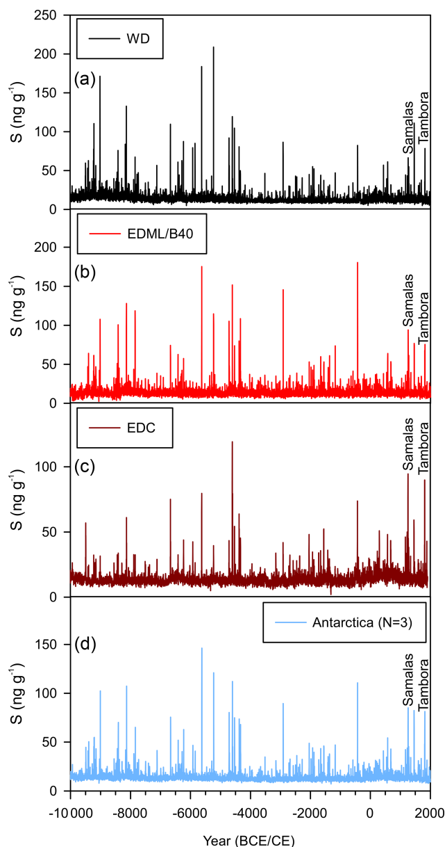
Figure 3. Holocene sulfur records from Antarctica: sulfur concentration records from the (a) WD, (b) EDML and (c) EDC ice cores as well as (d) a stack (“Antarctica” or ANT12k) of all three records for the Holocene (10 000 BCE–2000 CE). Measured as sulfate, the EDML and EDC records are synchronized on the WD2014 chronology (Sigl et al., 2016), annualized and scaled to the WD record. The upper part from EDML is based on the 200 m long B40 ice core drilled at the same site in 2012 (Sigl et al., 2015). Signals from two large historic eruptions, Tambora (1815) and Samalas (1257), are marked.
