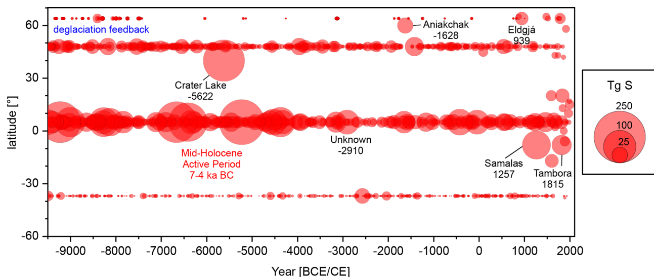
Figure 6. Spatiotemporal distribution of volcanic stratospheric sulfur injections from volcanic eruptions since 9500 BCE from HolVol 1.0 based on known and assigned locations (Iceland, 64° N; NHET, 48° N; tropics, 5° N; SHET, 37° S). Only eruptions with VSSI > 1 Tg S are included; prominent historic and prehistoric eruptions are marked; source attributions for Aniakhak and for Crater Lake are based on the geochemistry of cryptotephra from Greenland ice cores (Coulter et al., 2012; Zdanowicz et al., 1999).
