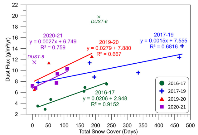
Fig. 8. Relation between duration of snow cover above a dust collector and dust flux during the winter seasons of 2016–17 and 2020–21, the 12-month interval from fall 2019 to fall 2020, and a long-duration collection spanning 2017–19. “DUST-6” and “DUST-8” mark individual samples excluded from the regressions because of local disturbance. In all cases a longer duration of snow cover corresponds to greater dust accumulation.
