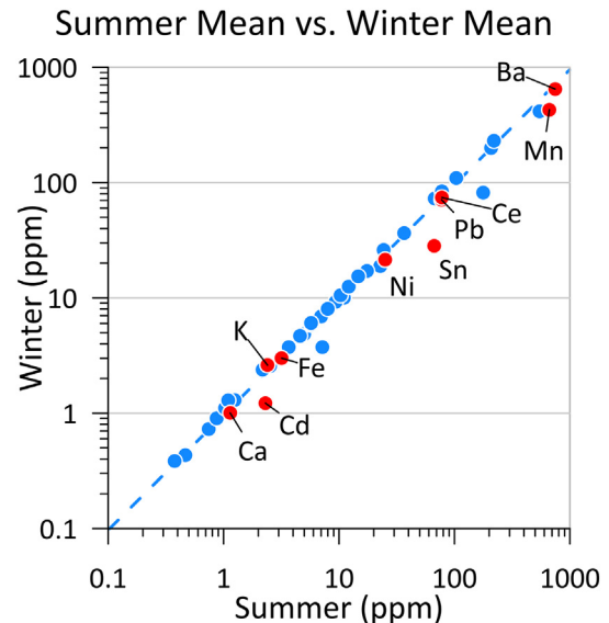
Fig. 6. Average values of major and trace elements in seasonal (winter/summer) pairs of Uinta dust samples. Elements plotted in red are significantly more abundant in summer (Ca, Cd, Fe, Ni, Sn, Pb, Ce, Mn, Ba) or winter (only K).
