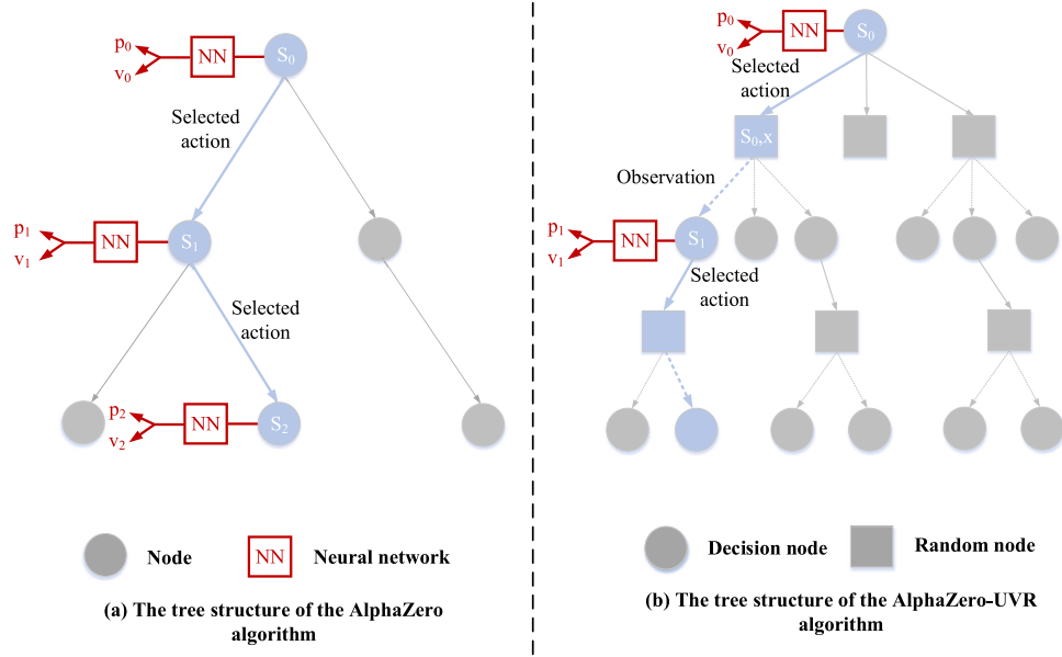
Fig. 4. Tree structure of the original AlphaZero algorithm [40] and the developed AlphaZero-UVR algorithm. The neural network takes system state as input and outputs action probabilities \mathbf{p} with components p_a = Pr(a|S) for each action a , and a scalar value v which represents the estimation of the expected outcome from the current state.
