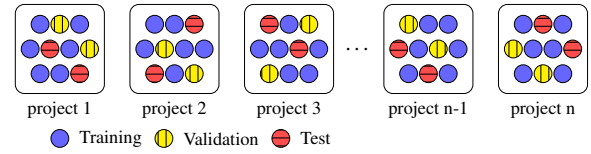
Figure 2: Mixed-project methodology.
