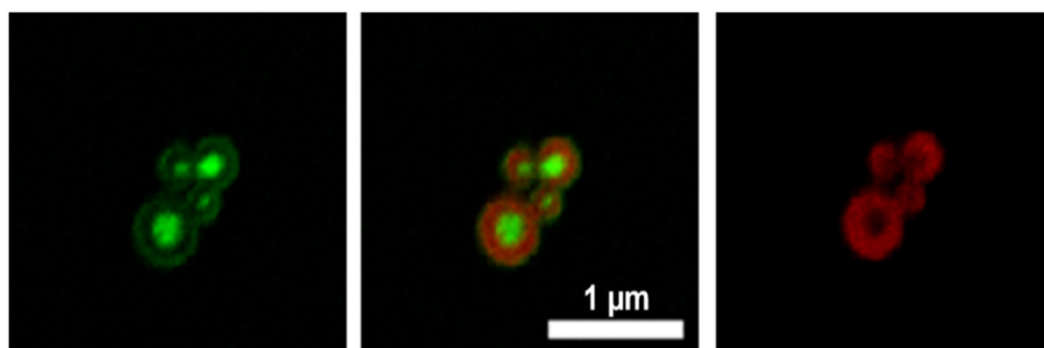
Figure 6. Representative confocal microscopy images for HByp4 with encapsulated 40 K MW dextrans. Fluorescein-labeled dextrans encapsulated mostly within the interior of the assemblies ( left ), with shells of the structures stained with Congo Red ( right ), and an overlap of both channels ( center ). Scale bar: 1 \mu m.
