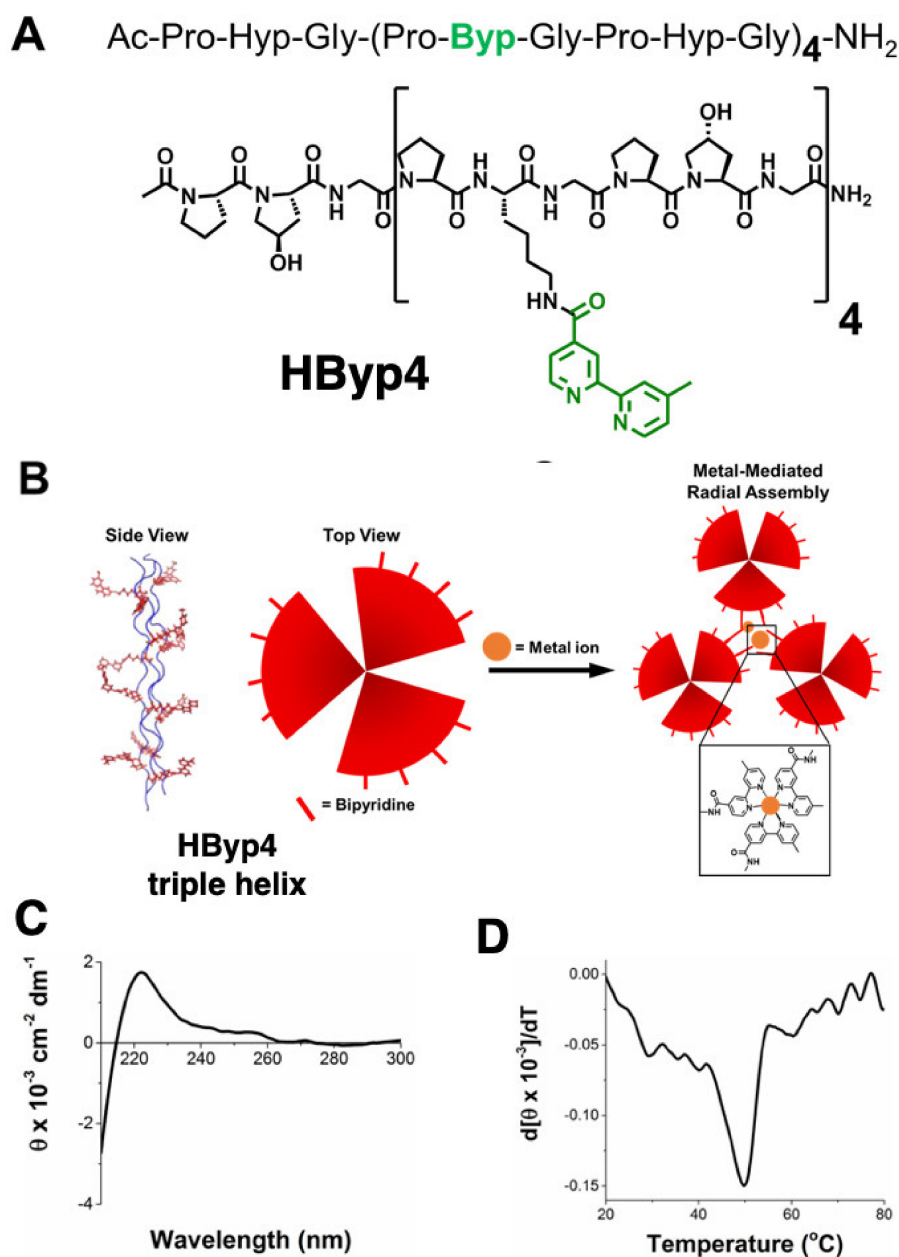
Figure 1. (A) The structure of HByp4; (B) metal ion-promoted assembly of the trimeric coiled coil; (C) CD spectrum of HByp4 (150 \mu\text{M} , 10 mM HEPES, pH 7.0); (D) first derivative of melting curve to determine the T_m value for HByp4.
