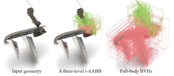
Fig. 2. i-AABB . Intersection-AABB (i-AABB) is a simple and more effective culling strategy than per-object BVHs often employed for rigid bodies. In this example, we collide helicopter and ship models with well over 343K surface triangles for the system. Culling with full-body BVHs leads to 1.3M AABB intersection tests. Instead, we build a shallow, three-level i-AABB based on the overlapping AABB volume, and the total number of intersection tests reduces to 120K, 90% fewer than regular BVH-based culling.
