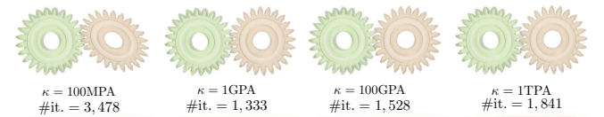
Fig. 9. ABD with different \kappa . We use ABD to simulate a pair of coupled gears under different \kappa values. The time step size is \Delta t = 1/100 sec, and \hat{d} = 0.001 m. A small \kappa leads to observable affine deformations. Increasing \kappa quickly eliminates this artifact. The convergence is lightly impacted by increased stiffness. Fortunately even if we set the \kappa 10 \times bigger than the default value of 100GPa, the convergence slow remains reasonable.
