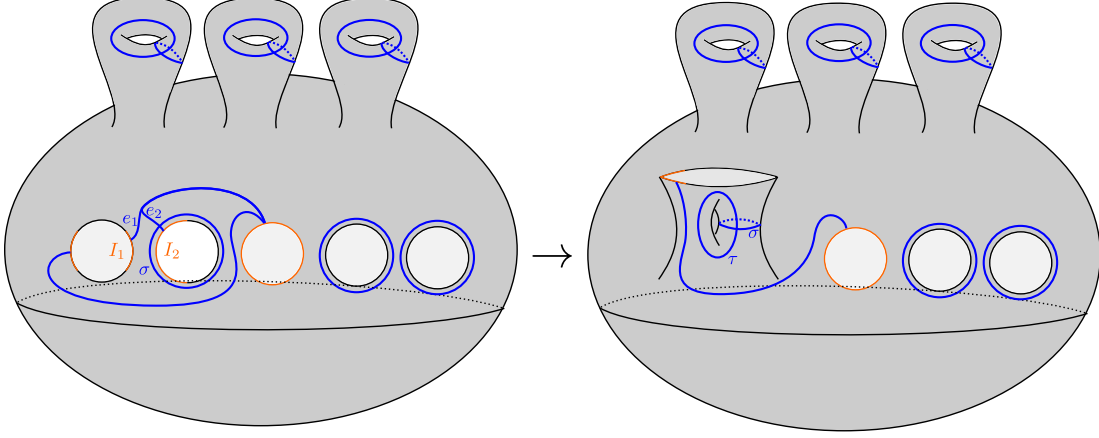
FIGURE 21. Left: F before gluing intervals I_1, I_2 on the same component of F but different components of \partial F . Right: the glued surface \bar{F} .
