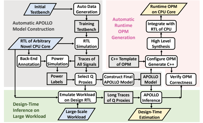
Figure 2: The automated APOLLO framework.
