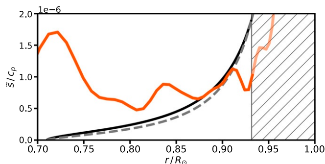
Fig. 5. Radial entropy profiles. The orange curve is the \theta rms of the two-dimensional profile from Fig. 4. The black curve is the convective estimate regime based on the flux debt; (2\Omega H_p F_0^3)^{1/5}/h_0 with background enthalpy h_0 = c_p T_0 . The dashed curve shows the estimate based on nonrotating theory, F_0^{2/3}/h_0 . By magnitude, all three of these profiles are consistent. Distinguishing rotating vs. nonrotating theories lies with other quantities, particularly the convective length scale.
