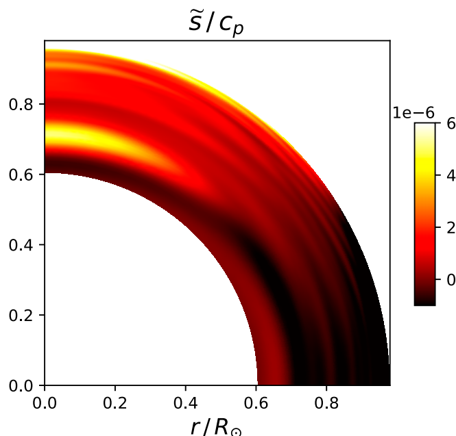
Fig. 4. The local thermal-wind entropy profile computed from helioseismic-inferred profile \Omega(r, \theta) in the convection zone. We use a fourth-order finite difference to compute \partial_z = \cos \theta \partial_r - r^{-1} \sin \theta \partial_\theta and a trapezoidal rule to integrate over \theta . The data are found in the electronic supplementary material from Larson and Schou (92).
