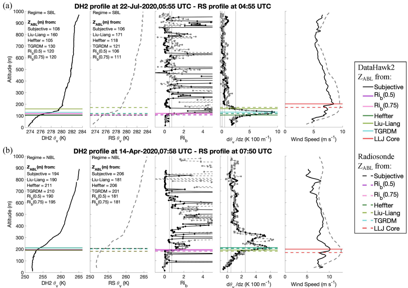
Figure 3. Demonstration of Z_{\text{ABL}} identification using all objective methods on both the DH2 (represented by solid lines) and corresponding radiosonde (represented by dashed lines) for an (a) SBL and (b) NBL case. From left to right the following profiles are shown: \theta_v profile from the DH2, \theta_v profile from the radiosonde, Ri_b profiles from the DH2 (solid black) and the radiosonde (dashed grey), d\theta_v/dz profiles from the DH2 (solid black) and the radiosonde (dashed grey), and wind speed profiles from the DH2 (solid black) and radiosonde (dashed grey). The legend on the right indicates the Z_{\text{ABL}} detection method associated with each horizontal line in the figure. The LLJ core is not in itself a Z_{\text{ABL}} detection method but plays into the Liu–Liang method, and thus it is included. Each Z_{\text{ABL}} is written on the corresponding platform’s \theta_v profile.
