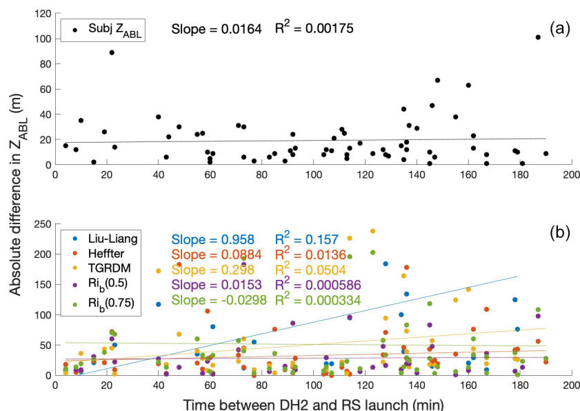
Figure 4. Absolute difference between subjective Z_{ABL} from the DH2 and subjective Z_{ABL} from the radiosonde closest in time to the DH2 launch (black dots, a ) and absolute difference between objective Z_{ABL} from the DH2 and objective Z_{ABL} from the radiosonde closest in time to the DH2 launch (colored dots, b ) versus absolute time difference in minutes between the DH2 and radiosonde launches. A few outlier points are not shown, as they lie outside the range of the y axis. Lines of best fit are included for the subjective Z_{ABL} and for each objective method, and the slope and R^2 value of each line is written next to the legend.
