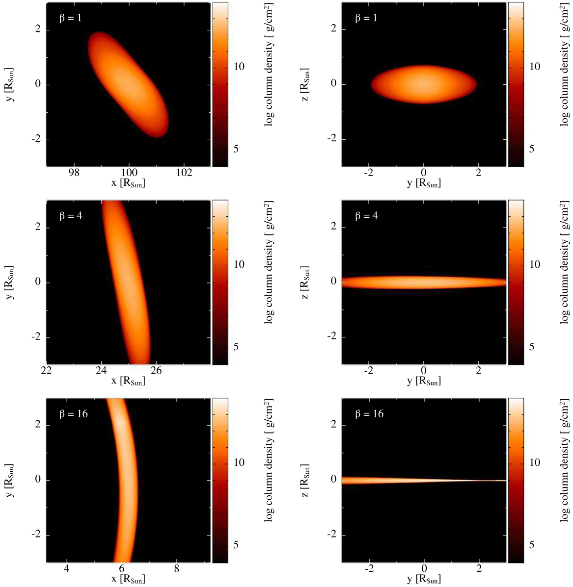
Figure 1. Column density renderings of the \beta = 1, 4 , and 16 simulations performed with 128M particles when the center-of-mass orbit for the star reaches pericenter. The left column shows the distribution in the orbital plane, and the right column shows the view across the orbital plane. The center of mass of the star starts in the negative x - and y -quadrant, and reaches pericenter with a positive x -position and y = 0 . Stellar material at positive y -values therefore has already passed pericenter, and negative y -values are yet to reach the pericenter of the original stellar orbit. The top panels correspond to \beta = 1 , the middle panels to \beta = 4 , and the bottom panels to \beta = 16 . In each case, we have restricted the view to the position of the center of mass \pm 3R_\odot , which for larger \beta does not quite encompass the entire debris stream, with larger \beta corresponding to more stretching of the star by the time pericenter is reached. As \beta is increased, the star is increasingly crushed into the orbital plane, with the thickness for \beta = 16 being \sim 0.01\text{--}0.1 R_\odot (the spread in vertical height is due to the fact that the point of maximum compression occurs slightly post-pericenter, and most of the star has not yet reached this point).
