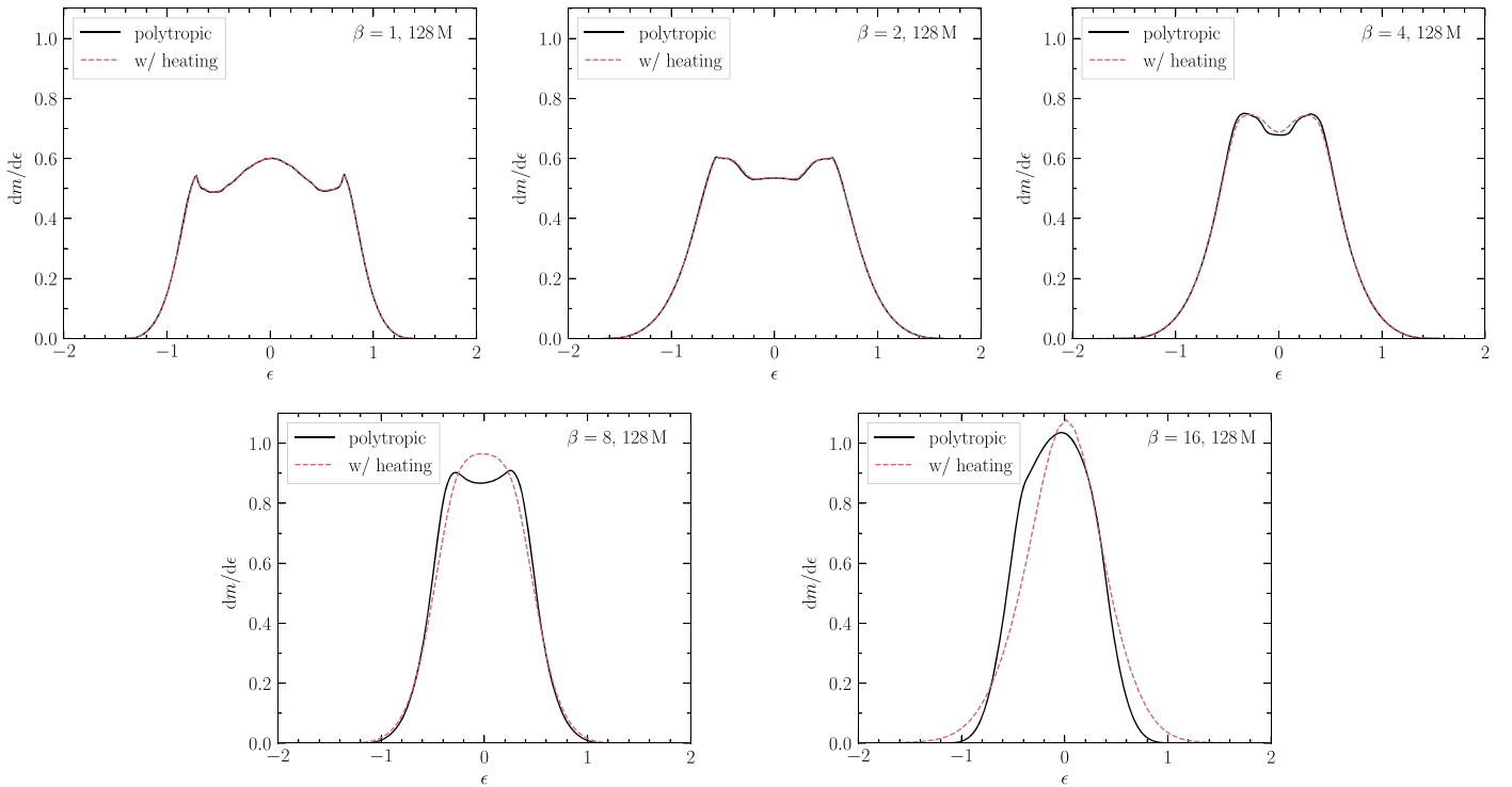
Figure 7. Energy distributions for the simulations with N_p = 128 M, comparing the effect of excluding (polytropic) and including heating of the debris (with heating). In each panel, the value of \beta is given at the top right of the panel. These energy distributions are calculated when the center-of-mass orbit has receded to a distance of 5r_t (e.g., Figures 3 and 4). The heating of the gas is mediated in the simulations by the numerical viscosity, which captures the heating due to shocks. Coughlin & Nixon (2021) showed that shocks should occur for \beta \gtrsim 3 , and that the shocks are typically weak, suggesting that their effect on the entropy of the gas is mild. This figure shows that the effect of shock heating on the energy distribution is typically small.
