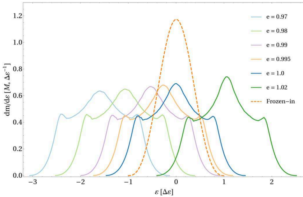
Figure 5. The differential mass per unit energy as a function of Keplerian energy, where the energy is in units of \Delta\epsilon = GM_* R_*/r_t^2 , and mass is in units of solar masses. The orange, dashed curve shows the prediction from the frozen-in approximation with e = 1 for comparison.
