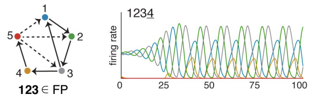
att 4 - pure tadpole (T graph) (7 graphs, 8 attractors)
