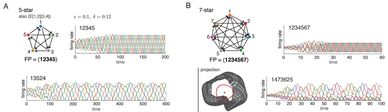
Fig 9. Symmetry can lead to spurious attractors. (A) Although the 5-star graph has only a single attractor in the standard CTLN parameters, for \varepsilon = 0.1 , \delta = 0.12 a second attractor emerges (bottom). Both can be accessed via small perturbations of the unique fixed point. (B) The 7-star graph also has two attractors that can be accessed from a single core fixed point, even in the standard parameters. The projection (bottom left) depicts a random projection of \mathbb{R}^7 onto the plane, with trajectories for the limit cycle (red circle) and an additional quasiperiodic attractor (black torus). The fixed point is also shown (red dot).
