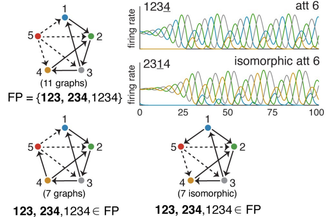
att 6 - pure F (18 graphs, 22+7=29 attractors)
