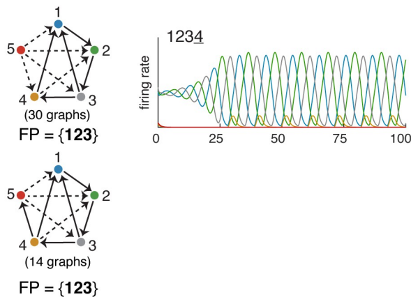
att 5 - pure D/E (44 graphs, 44 attractors)
