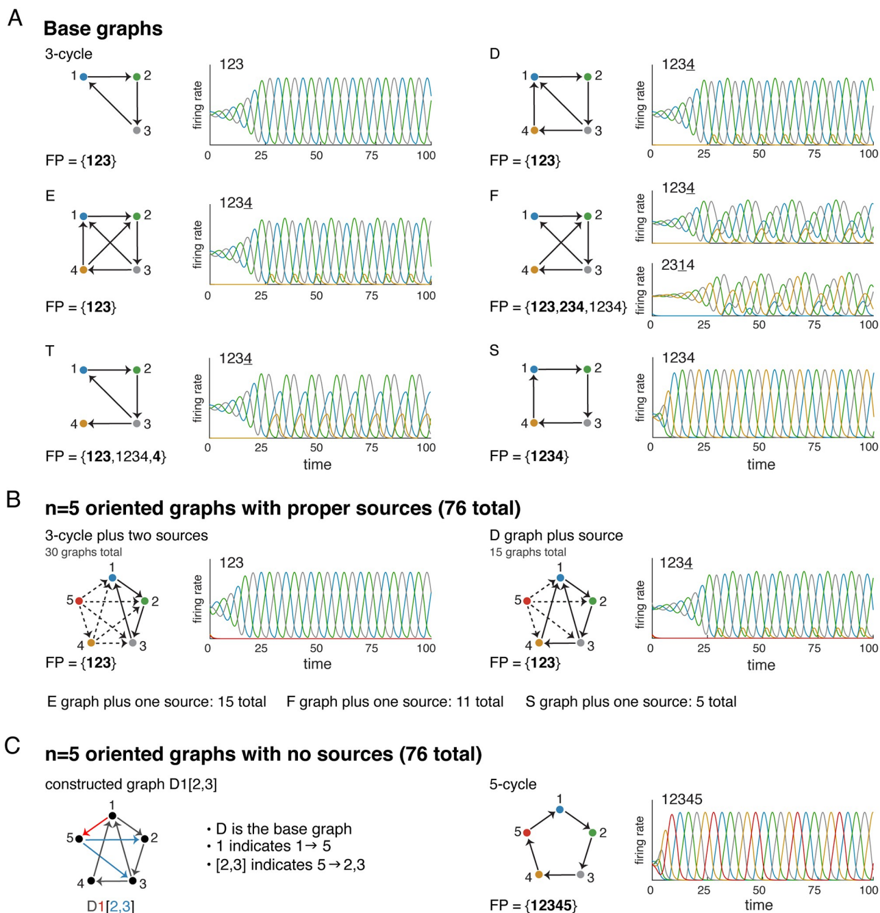
Fig 6. Taxonomy of n = 5 oriented graphs with no sinks. (A) Base graphs used to construct n = 5 graphs, and their corresponding attractors. Each attractor has a sequence, indicating the (periodic) order in which the neurons achieve their peak firing rates. (B) The oriented graphs with sources can be constructed by adding proper sources to each of the base graphs. This yields 30 graphs from the 3-cycle base (left), 15 graphs from the D graph base (right), and an additional 15, 11, and 5 graphs from the E, F and S graph bases. (C) All oriented graphs with no sources or sinks can be constructed from one of the D, E, F, T, and S base graphs. The graph label completely specifies the graph by naming the base and indicating the incoming and outgoing edges to the added node 5. (Left) For example, D1[2, 3] is the graph constructed from the D graph with added edges 1 \rightarrow 5 and 5 \rightarrow 2, 3 . (Right) The only oriented n = 5 graph with no sources or sinks that cannot be constructed in this way is the 5-cycle.
