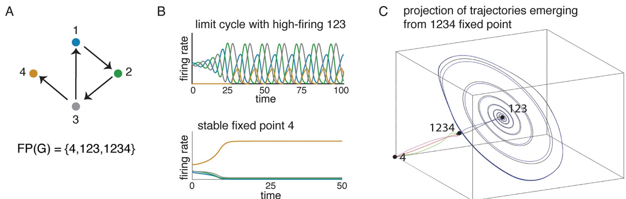
Fig 3. An example CTLN and its attractors. (A) The graph of a CTLN. Using graph rules, we can compute \text{FP}(G) . (B) Solutions to the CTLN with the graph in panel A using the standard parameters \theta = 1 , \varepsilon = 0.25 , and \delta = 0.5 . (Top) The initial condition was chosen as a small perturbation of the fixed point supported on 123. The activity quickly converges to a limit cycle where the high-firing neurons are the ones in the fixed point support. (Bottom) A different initial condition yields a solution that converges to the static attractor corresponding to the stable fixed point on node 4. (C) The three fixed points are depicted in a three-dimensional projection of the four-dimensional state space. Perturbations of the fixed point supported on 1234 produce solutions that either converge to the limit cycle shown in panel B, or to the stable fixed point. This fixed point thus lives on the boundary of the two basins of attraction, and behaves as a “tipping point” between the two attractors.
