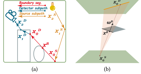
Fig. 2. Boundary segments: (a) A boundary light path is comprised of a boundary segment x_0^S x_0^D (shown in red) as well as a source and a detector subpath (illustrated in orange and blue, respectively). The two endpoints of the boundary segment are located on the visibility boundary of each other. (b) A boundary segment x_0^S x_0^D can be uniquely determined with a surface point x^B \in \mathcal{M} interior to the segment, along with a direction \omega^B .
