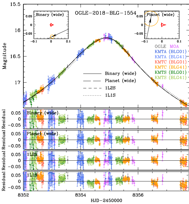
Fig. 11. Light curve and model for OGLE-2018-BLG-1554. The anomaly is characterized by weak deviations both before and after the peak. Like the previous two events, this one is subject to the Han & Gaudi (2008) planet/binary degeneracy (see insets), but even more severely (see Table 11). In addition, there is a severe 1L2S/2L1S degeneracy (see Table 11). Therefore, it is not established that the lens has a companion, and even if it does, this companion cannot be claimed as a planet.
