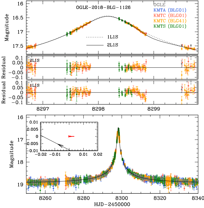
Fig. 1. Light curve and model for OGLE-2018-BLG-1126. The anomaly is a dip that is centered at 8298.7, which is detected at \Delta\chi^2 = \chi^2(1L1S) - \chi^2(2L1S) = 69 . As in all 10 light-curve figures in this paper, we show the full light curve and anomaly region in separate panels, we show the caustic topologies in one or more insets, we show residual panels for indicated models, and we color the data points by observatory, as indicated in the legend.
