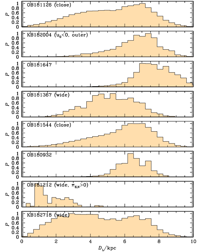
Fig. 15. Bayesian estimates of D_L for the 8 events shown in Table 13. Where there are several solutions, we show the distribution for the one with the lowest \chi^2 . However, as can be assessed from the Table 13, the other solutions hardly differ.
