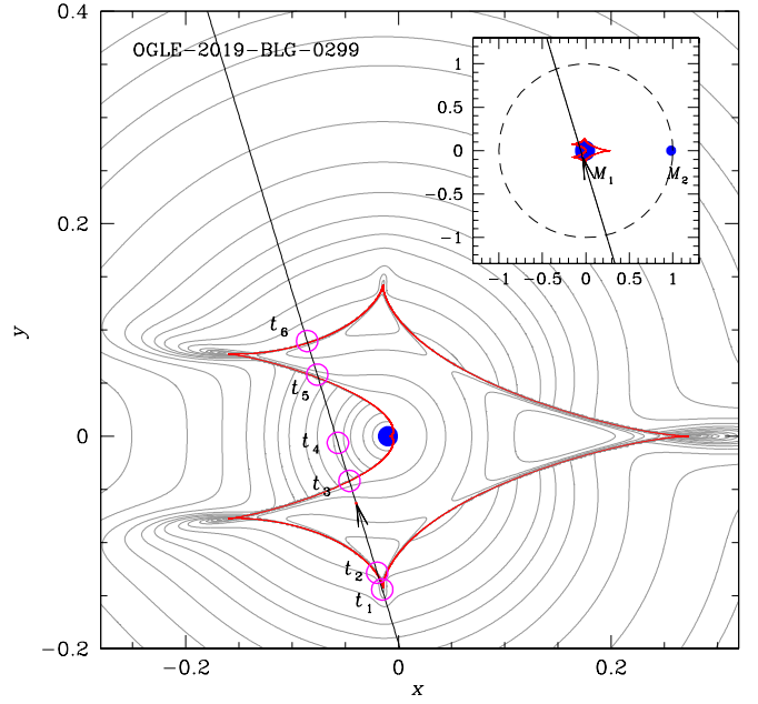
Fig. 10. Lens system configuration of OGLE-2019-BLG-0299. The empty magenta points represent the source positions corresponding to the six epochs of t_1 , t_2 , t_3 , t_4 , t_5 , and t_6 that are marked by arrows in Fig. 9. The size of the dots is not scaled.
