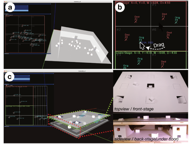
Figure 9: Control tool that visualize the real-time position of robots on the stages. (a: For the three wall stage in Figure 7a, b: Using a mouse cursor on the 2D view of GUI to specify the origin and destination points for each robot, c: Example of localization view with ramps and under-floor based on the design in Figure 7b. – the locations of robots on the software rendering and the actual setup are in sync.)
