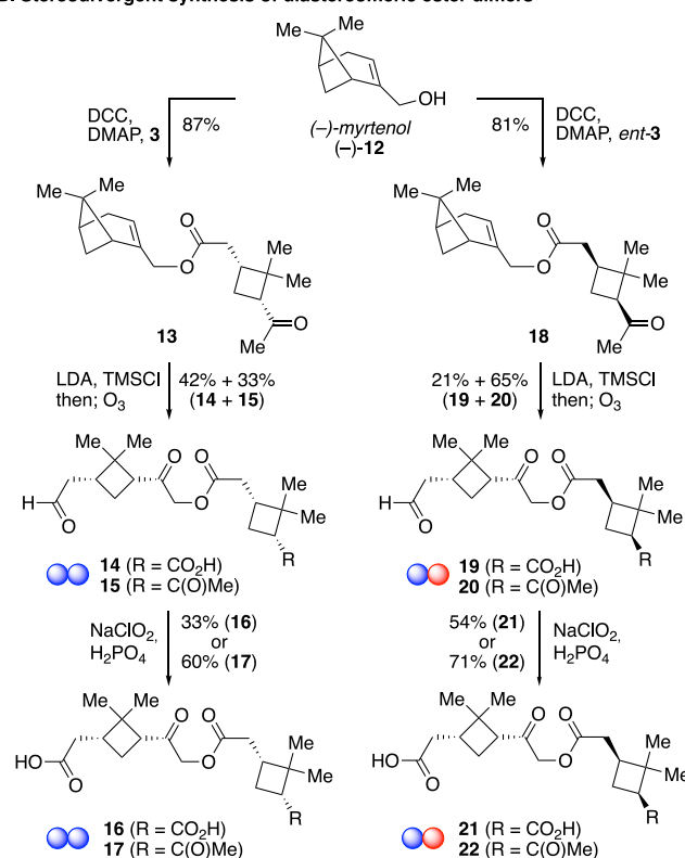
Figure 2. (A) Stereodivergent synthesis of the diastereomeric aldol dimers. (B) Stereodivergent synthesis of the diastereomeric ester dimers.
