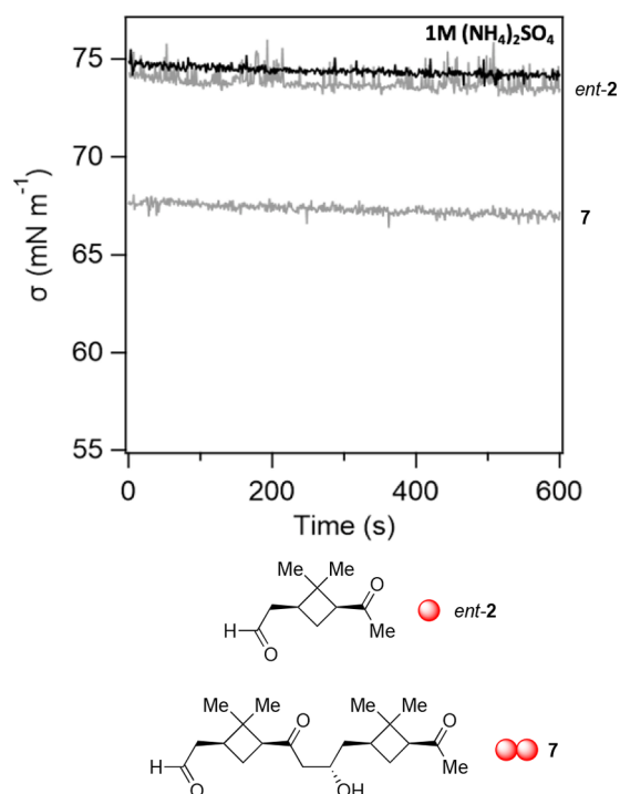
Figure 3. Surface tension ( \sigma ) over a 10 min period for ent -pinonaldehyde ( ent -2, top gray trace) and its aldol dimer (7, bottom gray trace) at 0.1 mM in 1.0 M (\text{NH}_4)_2\text{SO}_4 solution. The black trace shows the reference surface tension of 1.0 M (\text{NH}_4)_2\text{SO}_4 .
