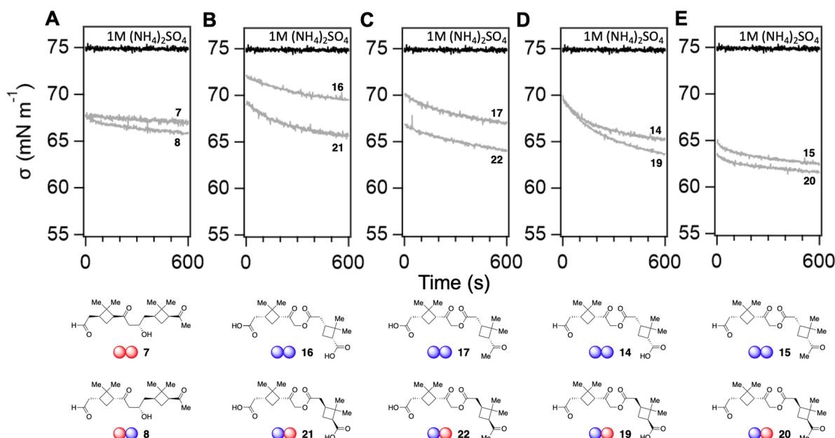
Figure 4. Surface tension ( \sigma ) over a 10 min period for each of the compounds shown. (A) Aldol addition dimers, (B) acid–acid ester dimers, (C) acid–ketone ester dimers, (D) aldehyde–acid ester dimers, (E) aldehyde–ketone ester dimers. Each compound was 0.1 mM in a 1 M (\text{NH}_4)_2\text{SO}_4 solution, and each trace is an average of 5–7 measurements. The black trace shows the reference surface tension of 1.0 M (\text{NH}_4)_2\text{SO}_4 .
