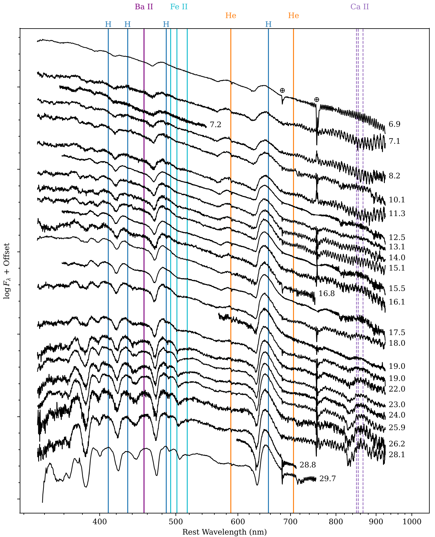
Figure 3. The spectroscopic evolution of SN 2011ja > 6 days after explosion, with colored lines at the rest wavelengths of selected features. (The data used to create this figure are available—See Figure 2.)
