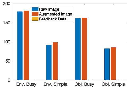
Fig. 13: Reported file sizes in kB when uploading to Firebase
