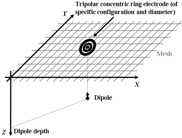
Figure 3. Schematic of the finite element method model used to compare Laplacian estimates.
