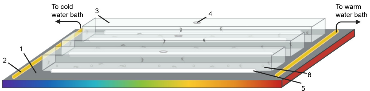
Figure 1. Schematic of the thermal gradient experimental setup. A temperature gradient was created on an aluminum plate (1) using a cold and a warm water bath on either side, connected with copper tubing (2). The mosquitoes were released into acrylic covers (3) through a hole in the top with a fitted acrylic plug (4). Each cover had moist wipe towels (5) and holes drilled on each side to minimize humidity build up (6). The acrylic enclosures are open on their bottom side to allow direct contact of mosquitoes with the aluminum plate.
