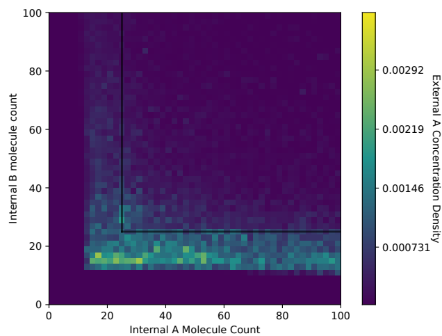
Figure 10. Heat map of the external A concentration with respect to A_{in} B_{in} for the adaptive receptor allocation strategy.
