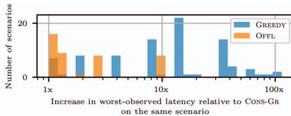
Fig. 3. We compare the worst-observed latencies for devices ( \tau_{x_i}, \tau_{x_j} ) on the harvesting scenarios \hat{h}_i, \hat{h}_j . Given an identical scenario, we find that CONS-GR outperforms both OFFL and GREEDY in terms of worst-observed latency by up to \sim 10x and \sim 100x respectively.
