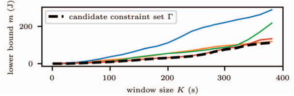
(b) Lower bound energy harvest versus window size computed by Eq. 1 Fig. 2. Energy harvesting traces with different behaviors can be captured with a single harvesting model. Here, historical wind harvesting data for the month of March across four years can be modeled with the candidate \Gamma -set shown in dashed black line in (b).
