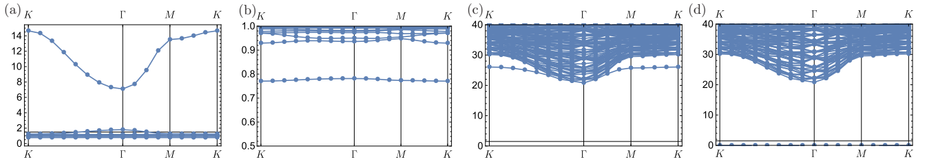
FIG. 7. Overlap matrix and trion bound states. (a) Spectrum of the inverse overlap matrix [\mathbb{1}_{N_M \times N_M} - \Delta^{(p,ey)}]^{-1} [Eq. (C10)] for \nu = 0 and double gate screening with \xi = 20 nm. (b) Zoomed-in spectrum below eigenvalue 1. (c) Spectrum of the projected trion Hamiltonian \tilde{H}^{(p,ey)} in Eq. (C13). (d) Spectrum of the matrix [\mathbb{1} - P(\mathbf{p})]\tilde{H}^{(p,ey)}[\mathbb{1} - P(\mathbf{p})] .
