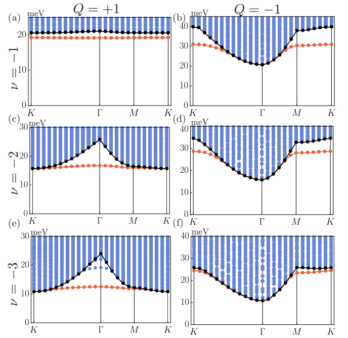
FIG. 3. Chiral limit trion spectra obtained after projecting the N = 3 scattering matrix into low-energy quasiparticle-Goldstone states, with minimum of quasiparticle-Goldstone continuum highlighted (black). See Fig. 2 for model parameters. For \nu = -1, Q = 1 [panel (a)], the trion bound state persists at all momenta (but due to its small binding energy likely disappears outside the chiral limit).
