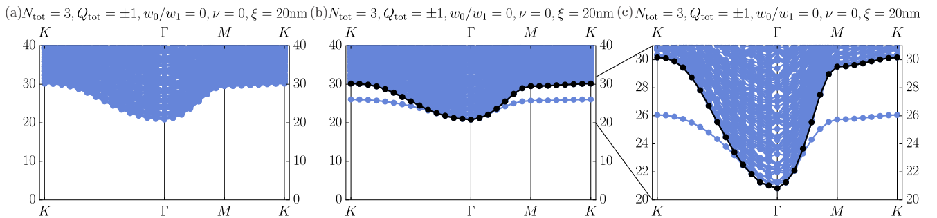
FIG. 6. Quasiparticle-Goldstone and trion spectra. (a) Free quasiparticle-Goldstone continuum. (b) Spectrum of the chiral limit trion scattering matrix in Eq. (C13) for equal chiral sectors ( e''_Y = e'_Y = e_Y ), with minimum of the quasiparticle-Goldstone continuum highlighted. (c) Enlarged trion spectrum. A trion bound state develops away from the \Gamma point of the mBZ.
