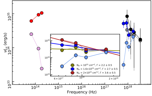
Fig. 5. Main panel: comparison between observed and corrected spectra. The cyan, gray, and pink points show the spectra as observed by Chandra, NuSTAR, and in the IR band, respectively. The blue, black, and red points show the same data corrected for absorption and the effects of dust scattering. The correction amounts to more than one order of magnitude in K and H as well as in the soft X-ray band. Inset: as in the main panel, the cyan points show the spectrum as observed by Chandra. The olive, blue, and dark red points show the Chandra spectrum after correction assuming N_{\text{H}} = 10^{23} , 1.6 \times 10^{23} , and 2 \times 10^{23}\text{ cm}^{-2} , respectively.
