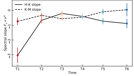
Fig. 6. Infrared spectral slopes \alpha for the six times T1 to T6. The color encodes the time, dark red to dark blue. The black solid line shows the H – K slope; the black dashed line shows the K – M slope.
