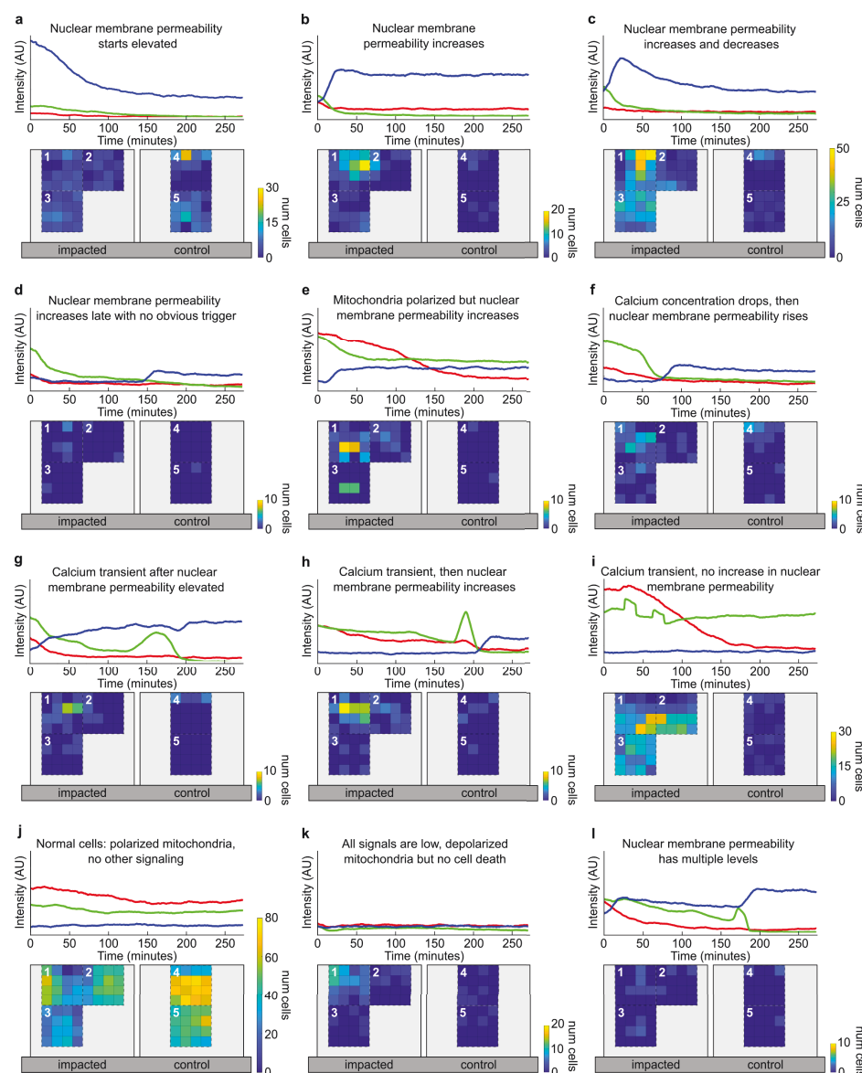
FIG. 4. Cell behavior categories and their distributions. For each category, a representative time series for a single cell (top, with blue representing nuclear membrane permeability, green representing calcium concentration, and red representing mitochondrial polarity) along with a heat map of cell counts indicating relative frequency at different locations are shown. Colorbar maxima vary between categories to resolve spatial distributions for categories with fewer cells. Regions 1-3 are on the impacted sample, with 1 as the site of impact. Regions 4-5 are on the control sample. a) The nuclear membrane permeability starts out elevated and decays. b) The nuclear membrane permeability increases within 30 min of impact and plateaus or continues increasing. c) The nuclear membrane permeability increases within 30 min of impact and then decays. d) The nuclear membrane permeability increases after 30 min after impact but no prior signaling event is observed. e) The nuclear membrane permeability increases despite the mitochondria being polarized. f) The nuclear membrane permeability increases after the calcium concentration drops after a period of sustained elevation. g) Transient calcium signaling is observed after the nuclear membrane permeability has already increased. h) The nuclear membrane permeability increases after calcium transient(s). i) Calcium transient(s) are observed with no increase in nuclear membrane permeability. j) No calcium transients or increases in nuclear membrane permeability. k) All three signals are very low. l) The nuclear membrane permeability increases multiple times.
