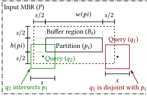
Figure 4: Relationship of a range query with a partition
