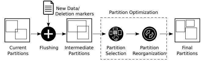
Figure 3: Overview of the proposed framework
