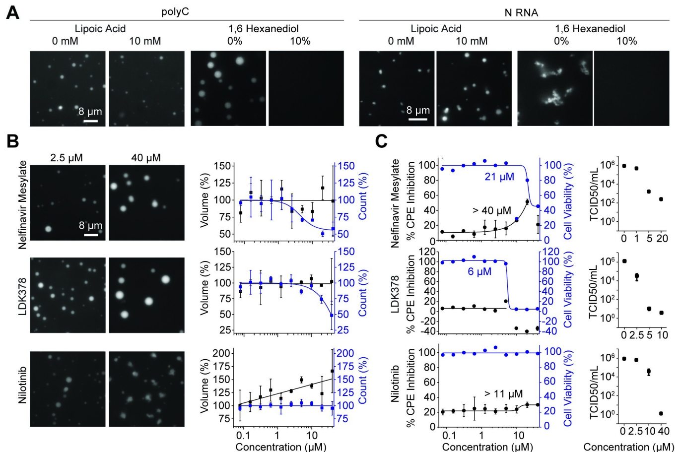
Fig 5. Identification of small molecules that alter phase separation of N in vitro and reduce viral titer in SARS-CoV-2 infected cells. (A) Condensates formed in the presence of 7.8 μM N and either 50 ng/μL polyC or 18 nM 0–5 kb viral RNA were not affected by 10 mM lipoic acid but dissolved in the presence of 10% 1,6 hexanediol. (B) (Left) Examples of drugs that affected N phase separation with polyC in vitro. The N protein and polyC RNA concentrations were set to 7.8 μM and 50 ng/μL, respectively. (Right) The percent change on the number (blue) and total volume (black) of N-polyC condensates settled per micron squared area on the coverslip under different drug concentrations (mean ± SD, n = 8 with 2 technical replicates). Solid curves represent a fit to a dose-response equation (see Methods ). (C) (Left) Percent CPE inhibition (black, mean ± SD, 2 technical replicates) and cell viability (blue) of SARS-CoV-2-infected Vero-E6 cells treated with serial dilutions of drugs. Solid curves represent a fit to a dose-response equation (see Methods ) to determine a half-maximal response constant EC_{50} ( S4 Table ). (Right) Viral titer in SARS-CoV-2-infected Vero-E6 cells treated with serial dilutions of drugs as measured by a TCID 50 assay (mean ± SD, 3 technical replicates). Data underlying this figure can be found in S1 Data . CPE, cytopathic effect; N, nucleocapsid; SARS-CoV-2, Severe Acute Respiratory Syndrome Coronavirus 2; TCID, tissue culture infectious dose.
