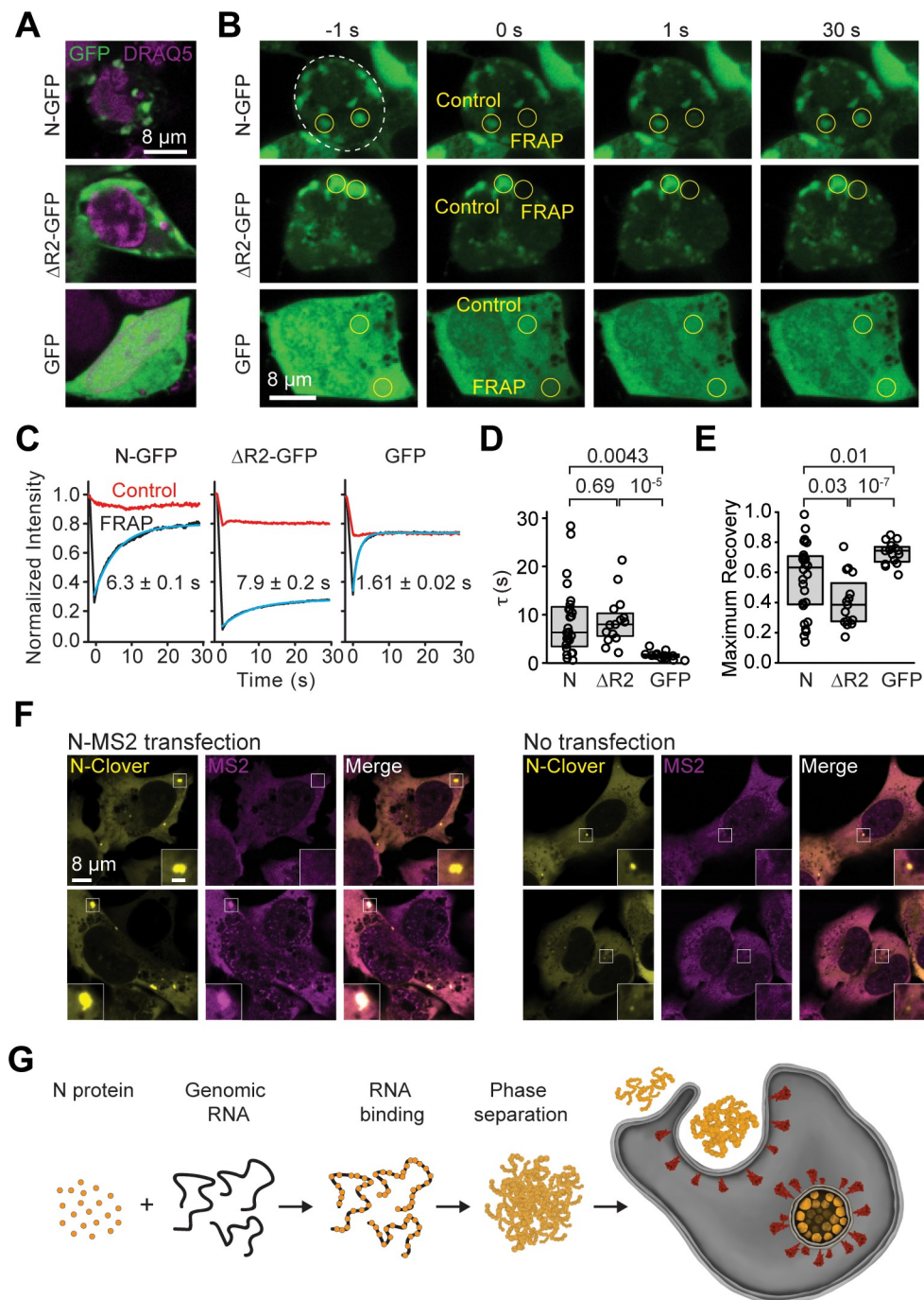
Fig 6. Dynamics of N condensates in vivo. (A) Example images of HEK293T cells expressing N-GFP, ΔR2-GFP, and GFP stained with DRAQ5. (B) Representative FRAP imaging of cells exhibiting N-GFP or ΔR2-GFP puncta or high GFP expression. Circles show the photobleached area. (C) Fluorescence recovery of the GFP signal in the bleached versus the control regions. The solid curve represents a single exponential fit to reveal the recovery lifetime ( \tau , \pm 95\% confidence interval). (D) The distribution of fluorescence recovery lifetimes of cells expressing N-GFP ( n = 28 ) or ΔR2-GFP ( n = 15 ) exhibiting puncta and GFP only ( n = 15 ). The center and edges of the box represent the median with the first and third quartiles. The p -values were calculated from a 2-tailed t test. (E) The maximum fractional recovery after photobleaching of cells expressing N-GFP ( n = 28 ), ΔR2-GFP ( n = 15 ), or GFP only ( n = 15 ). The center and edges of the box represent the median with the first and third quartiles. The p -values were calculated from a 2-tailed t test. (F) U2OS cells stably expressing N-Clover form condensates in the cytoplasm. (Left) Cells co-transfected with an N-MS2 expression plasmid exhibit colocalization of N-Clover and Cy3-MS2 FISH signal in N-condensates ( N = 10 out of 55 cells, 2 technical replicates). (Right) The Cy3-MS2 FISH probe does not partition into N condensates
