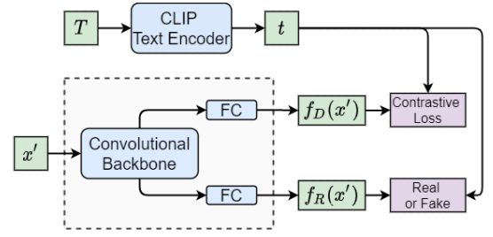
Figure 3: Illustration of the proposed discriminator. FC denotes fully-connected layers.
