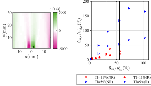
Fig. 3: Coherent velocity response in the shear layer as a function of in-flow forcing input for both turbulence conditions for reacting (R) and non-reacting (NR) flows.
