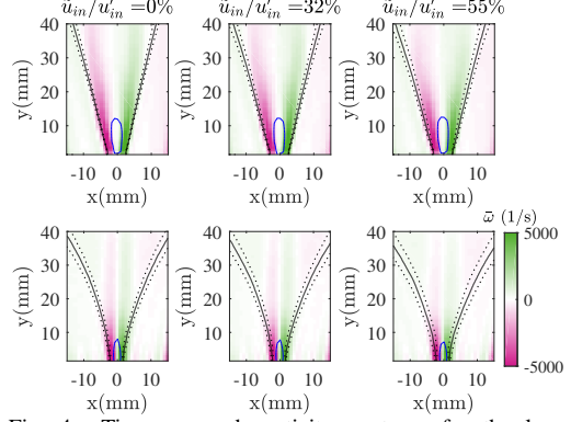
Fig. 4: Time-averaged vorticity contours for the low-turbulence (top row) and high-turbulence (bottom row) conditions. The black solid line depicts the mean flame edge ( \bar{c} = 0.5 ) and the dotted lines represent the \bar{c} = 0.3 and \bar{c} = 0.7 contours. The blue contour represents the limits of recirculation zone, \bar{u}_y = 0 .
