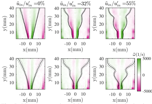
Fig. 5: Phase-averaged vorticity contours at a single phase for the TI = 5\% (top row) and the TI = 11\% (bottom row) conditions ( \Phi = 180^\circ ). The solid black lines depict the phase-averaged \bar{c} = 0.5 contour and the dotted lines represent the phase-averaged \bar{c} = 0.3 and \bar{c} = 0.7 contours. (Videos of these conditions are available in the supplementary material.)
