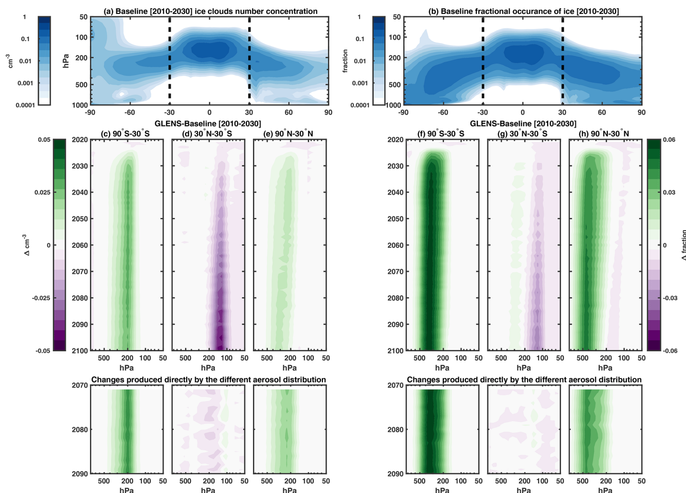
Figure 5. Baseline concentration of cloud ice number concentration ( a , number of particles per cm -3 ) and fractional occurrence ( b ) for the period 2010–2030. In panels ( c )–( e ) and ( f )–( h ), the yearly evolution of the differences between GLENS and Baseline (in the 2010–2030 period, as for the panels above) are shown for the three latitudinal boxes separately. In the small bottom panels, the effects of the changes produced by the aerosols are isolated by plotting the difference between GLENS and the simulations with surface cooling and stratospheric heating but no aerosols.
