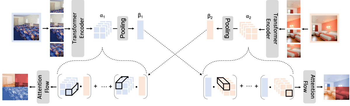
Figure 3. The top row shows the typical forward pass for an Transformer trained for image embedding. We highlight the tokens generated in the last block, \alpha , and the post-pooled feature vector, \beta . The similarity between two feature vectors, typically computed as \frac{\beta_1}{\|\beta_1\|} \cdot \frac{\beta_2}{\|\beta_2\|} , can be spatially decomposed using the approach described in Section 3, resulting in a pair of heatmaps that highlight the input regions in each image that most contributed to the similarity with the other image.
