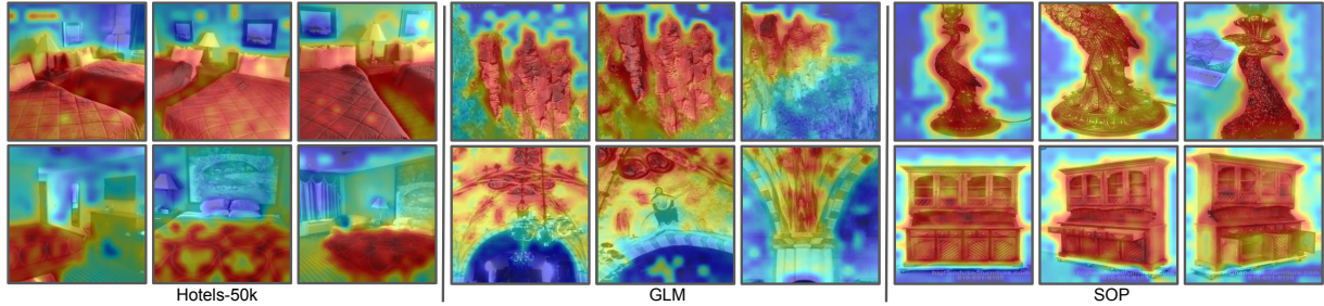
Figure 5. Class similarity maps from selected images. All images in a given row belong to the same class.
