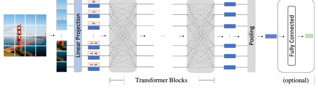
Figure 2. Our visualization approach is applicable to Transformers whose input is non-overlapping image patches with varying numbers of encoding blocks followed by a pooling layer (and perhaps a fully-connected layer) to generate the output feature, such as Swin [23], HVT [24], and PSViT [9].
