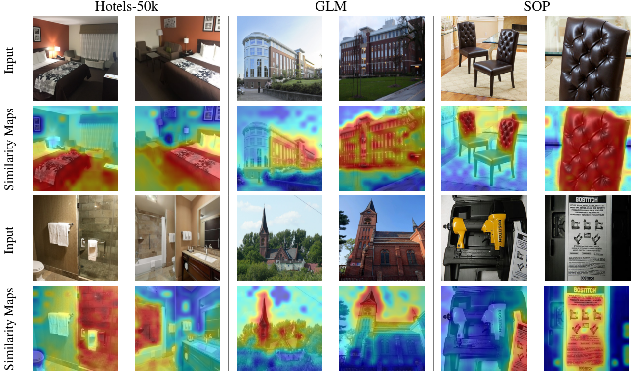
Figure 4. Paired image similarity maps for examples from the Hotels-50k, GLM, and SOP datasets.
