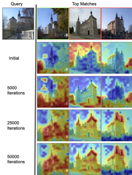
Figure 6. A query image and its top 3 matches, along with their accompanying similarity maps at different stages of training. A green border indicates a correct retrieval.
