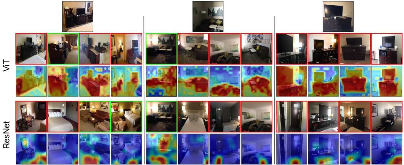
Figure 9. Image retrieval queries on Hotels-50k dataset (top row) and their the top-4 retrieved results for the ViT and the ResNet, along with their similarity maps computed with respect to the query. A green border indicates a correct retrieval.
