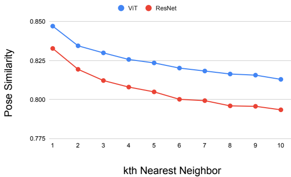
Figure 10. On average, the top matching images from a Transformer model have higher similarity of objects and camera pose to the query than for the ResNet, which suggests the presence of common objects contributes more strongly to similarity for Transformers than ResNets.
