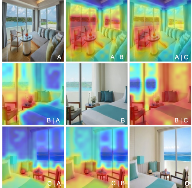
Figure 1. Our approach visualizes paired image similarity in Transformer networks trained for image embedding. For the images along the diagonal, the off-diagonal visualizations show the pairwise similarity maps generated by our approach, where red indicates a high contribution. For example, for image B , B|A , shows that the chair region contributes the most similarity with image A , while B|C also includes the bed and wall contributing to the similarity with image C .
