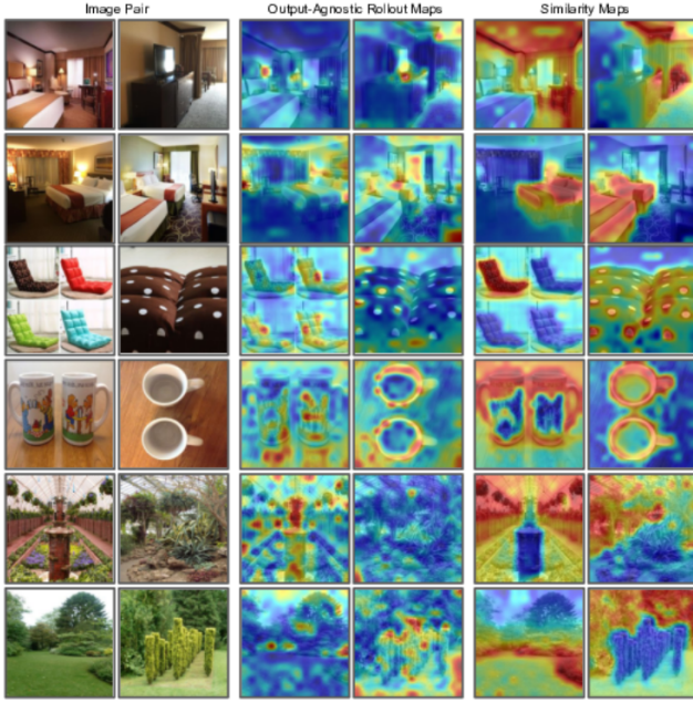
Figure 8. For a pair of images, output-agnostic Rollout maps and their corresponding similarity maps generated with respect to each other. In the Rollout maps, red regions have higher relevancy; in the similarity maps, red regions contribute more to the similarity.
