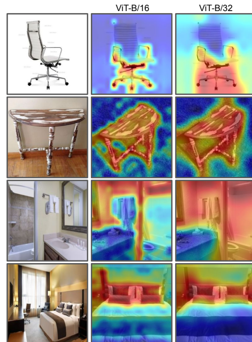
Figure 7. Similarity maps of the images in the center and right columns computed with respect to the image on the left. Smaller patch-size causes noisy fluctuations in similarity of the background regions. Larger patch-size causes the similarity of smaller objects to be influenced by that of larger, surrounding regions.
