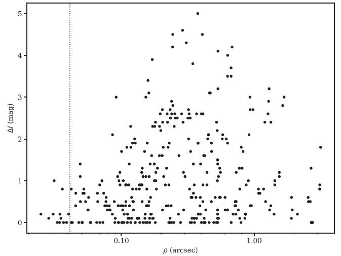
Figure 2. Separation \rho in arcsec and magnitude difference in I band for each observation that resolved a companion, excluding those for which the data were exceptionally noisy (“.” flag in Table 2). The 41 mas formal diffraction limit of SOAR is indicated with the vertical dotted line. This sample is intentionally focused on the closer pairs ( \lesssim 1'' ) that are more likely to show orbital motion over our 3 yr campaign.
