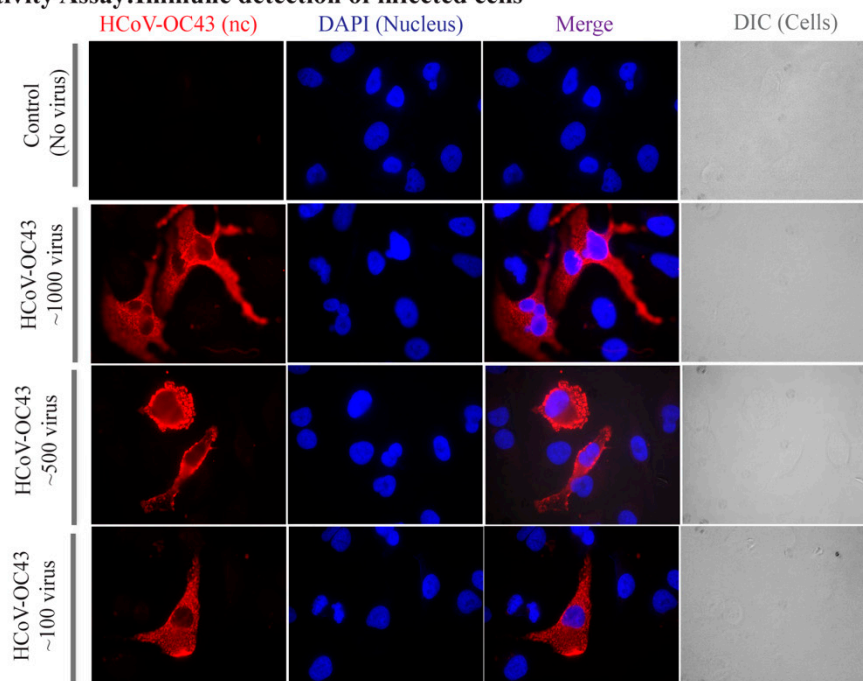
Figure 2. Assay establishment: Integrated cell culture PCR and Immune detection of HCoV-OC43 infected cells. (A). Standard curve of varying HCoV-OC43 genome copies with Ct value. (B). Correlation of HCoV-OC43 viral copies added onto A549-hACE2 cells and detection of intracellular viral genome copies following infection and replication. (C). Immune localization of HCoV-OC43 nucleocapsid protein in A549-hACE2 cells infected with varying amounts of virus. Nucleocapsid was detected with anti-HCoV-OC43 antibody followed by staining with chicken anti-mouse Alexa Fluor 594 (red). Nuclei were stained with DAPI (blue). DIC images are to show cell morphology.
