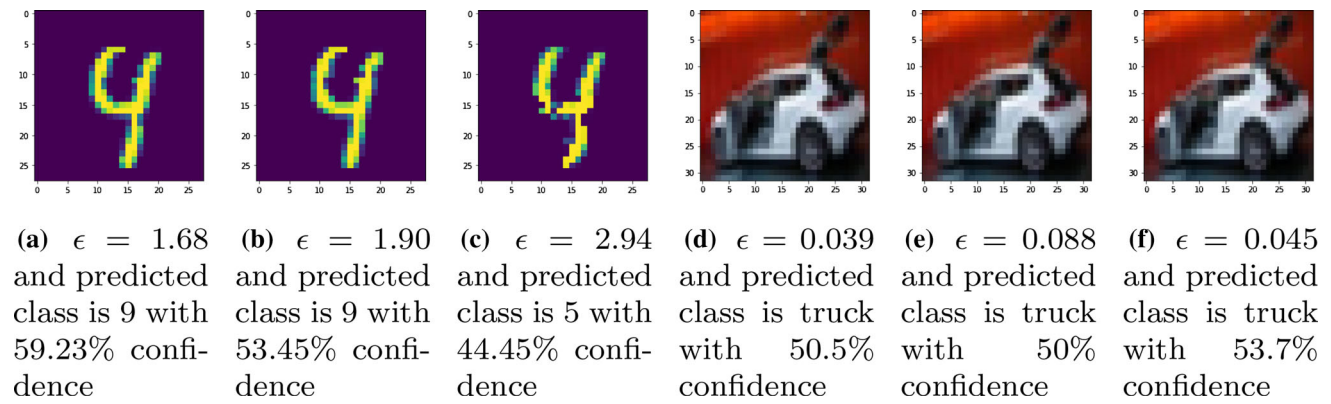
Fig. 7 CWA applied on a, d complete images, b, e top halves of images and c, f bottom halves of images
