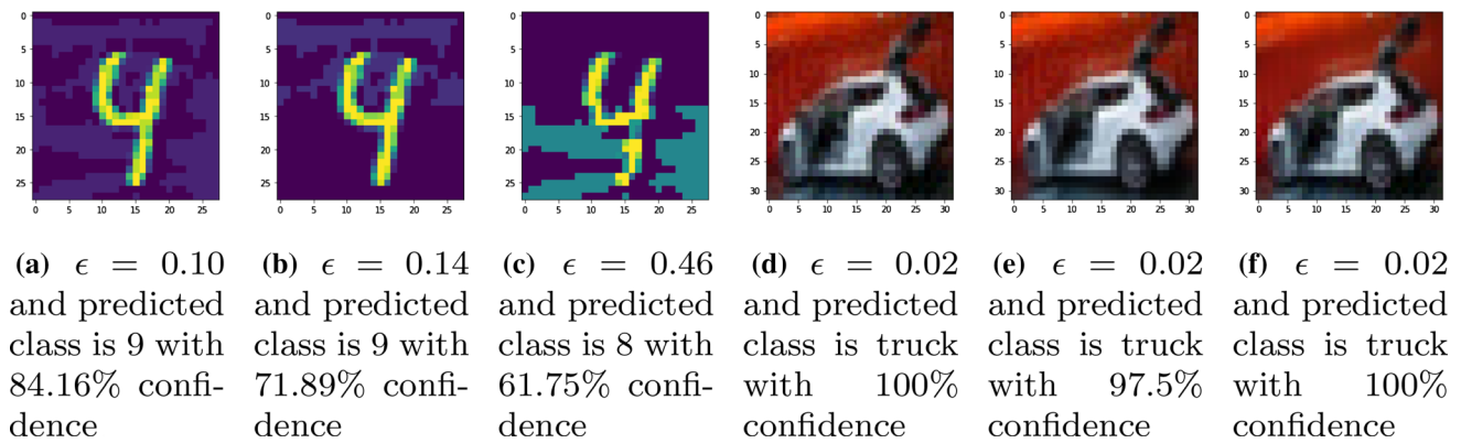
Fig. 5 FGSM applied on a, d complete images, b, e top halves of images and c, f bottom halves of images
