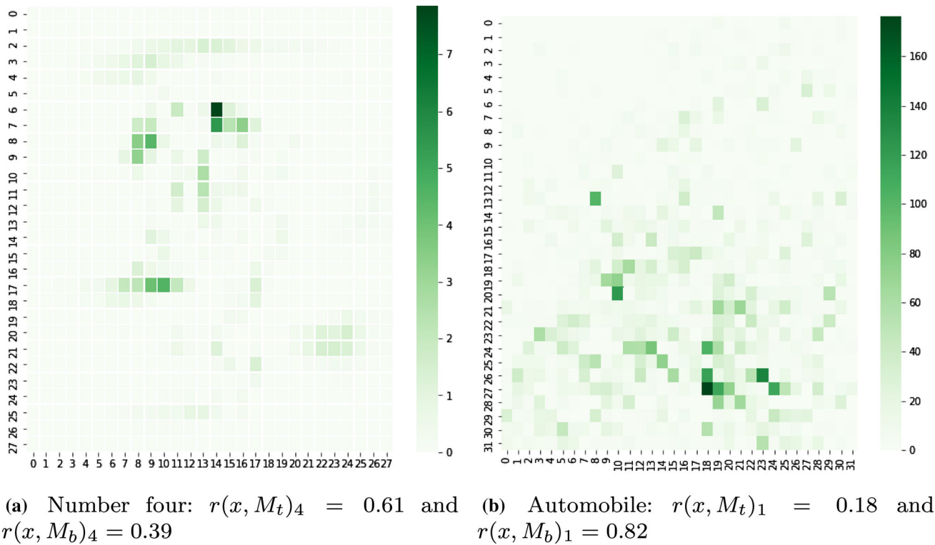
Fig. 11 Sensitivity maps: a the top half appears to have more sensitive regions; b shows sensitivity near the bottom half
