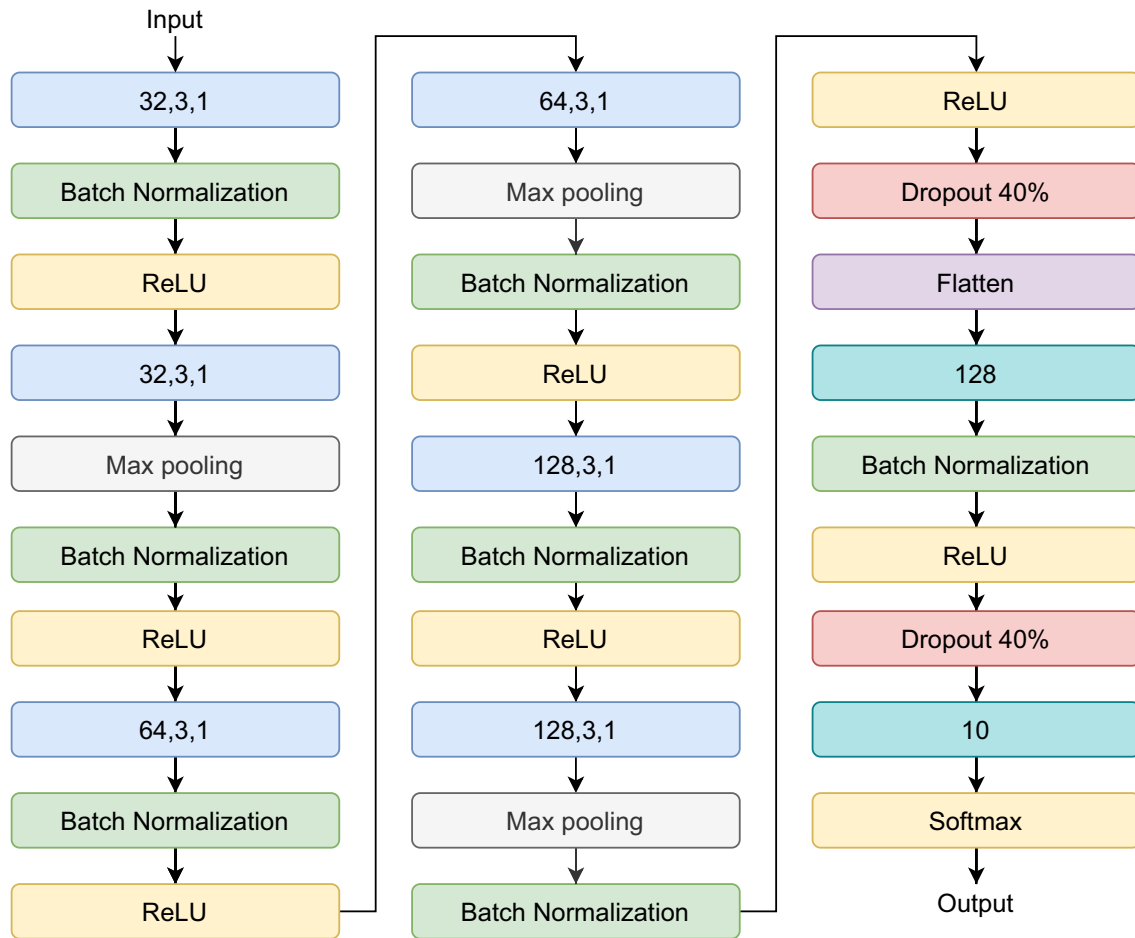
Fig. 13 Architecture of our CIFAR-10 classifier. Note that a dense layer and a convolutional layer are defined in the red rectangle in Fig. 12
