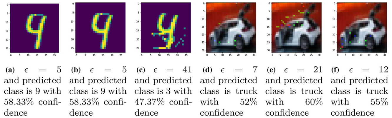
Fig. 8 JSMA applied on a, d complete images, b, e top halves of images and c, f bottom halves of images
