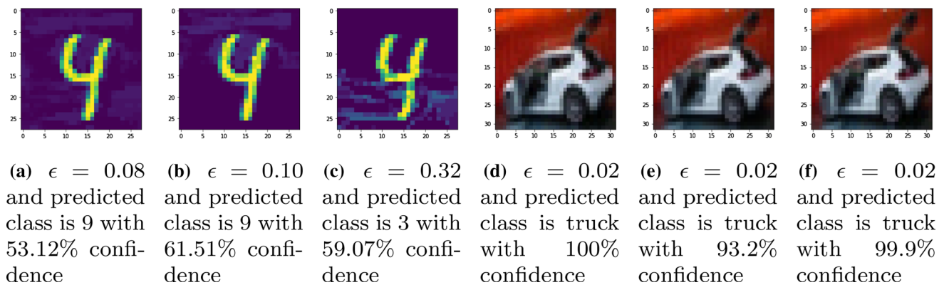
Fig. 6 IGSM applied on a, d complete images, b, e top halves of images and c, f bottom halves of images
