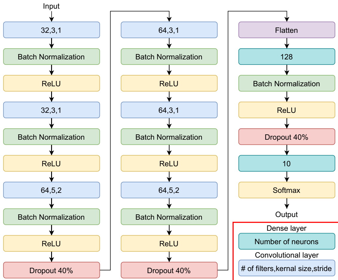
Fig. 12 Architecture of our MNIST classifier. Note that a dense layer and a convolutional layer are defined in the red rectangle
