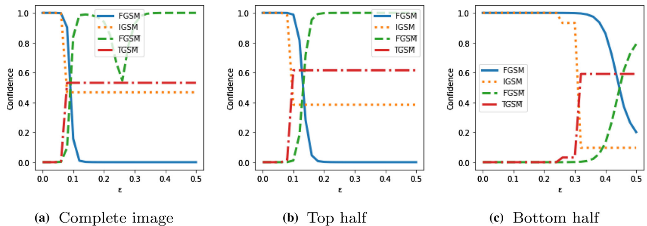
Fig. 9 These graphs summarize the confidences of number four and the highest-confidence class excluding number four over \epsilon
