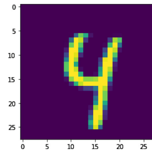
Fig. 3 Clean image of number four with 100% confidence classified by our MNIST classifier
