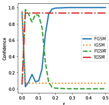
Fig. 10 This graph shows the confidences of automobile and the highest-confidence class excluding automobile over \epsilon where only top half is allowed to perturb
