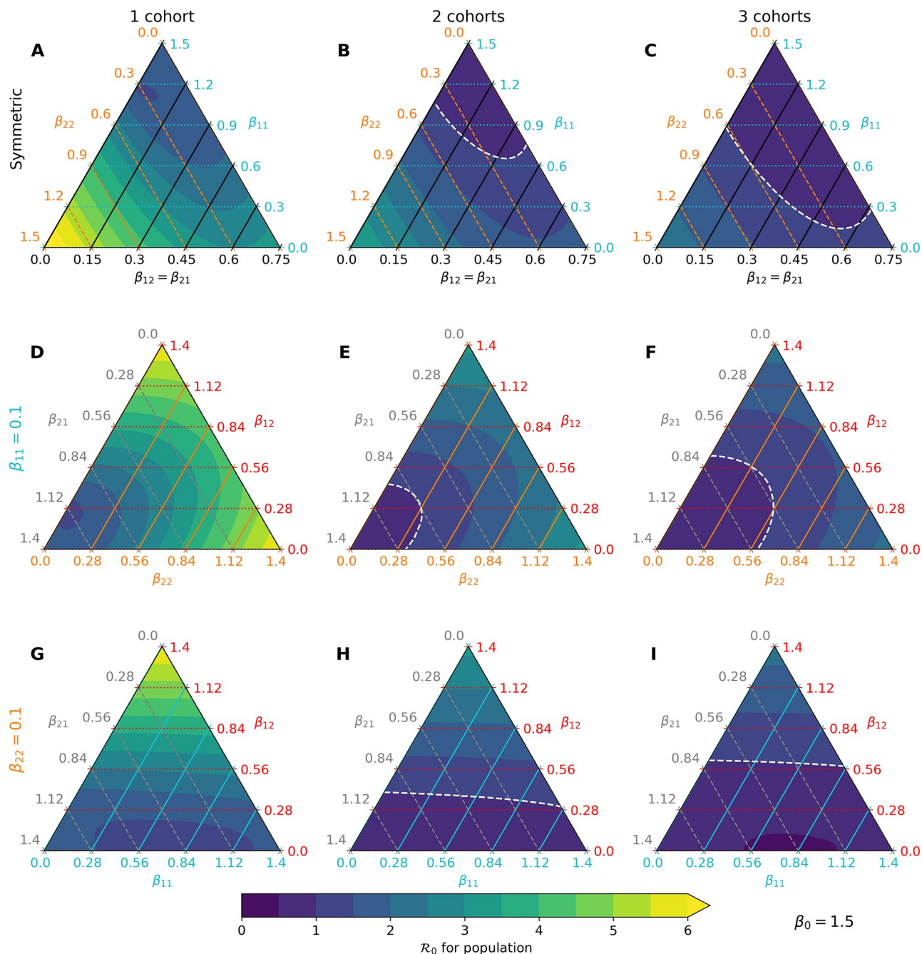
Fig 2. Predicted R_0 under various transmission-cohort scenarios. The color gradient changes from purple to blue to reflect R_0 shifting from < 1 to > 1 in each ternary plot, with the white line denoting the boundary. Yellow is used to represent R_0 > 6 . (A-C) Assuming child-adult and adult-adult transmission rates are identical (black axis), movement along the blue axis indicates that child-child transmission has a weak effect on R_0 at a fixed scale for \beta_0 . (D-F) Fixing child-child transmission to be weak ( \beta_{11} = 0.1 ) relative to other interactions, both child-adult and adult-adult transmission play dominant roles in increasing R_0 . (G-I) Fixing adult-adult transmission to be weak ( \beta_{22} = 0.1 ), only child-adult transmission plays a dominant role in increasing R_0 .
