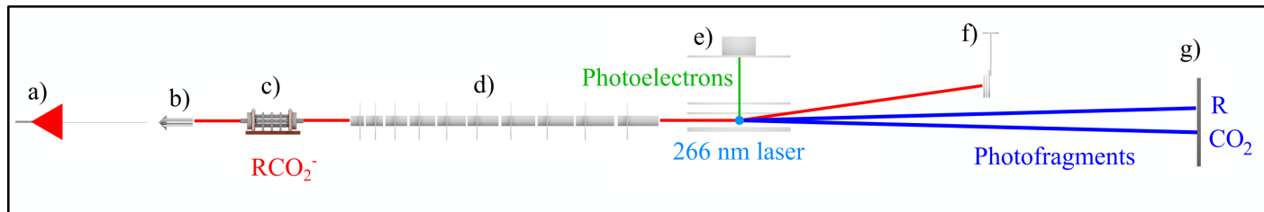
Fig. 1 Schematic of the high beam energy PPC spectrometer depicting the a) ESI source, b) octopole ion guide, c) hexapole accumulation trap, d) LINAC, e) electron detector, f) undetached ion deflector and g) neutral detector. 24 The 4.66 eV DPD of \text{RCO}_2^- is also shown.
