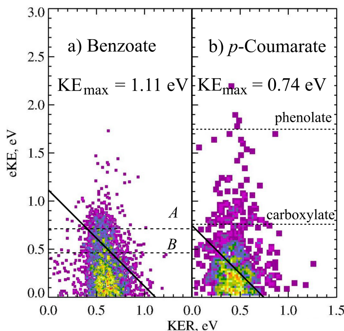
Fig. 5 The PPC spectrum for decarboxylation of 11 keV benzoate and p -coumarate recorded at 4.66 eV. The calculated KE_{\max} are depicted by the solid diagonal lines. The ADEs for photodetachment of benzoate to the A and B radical states and VDEs of the carboxylate or phenolate p -CA − to the corresponding radicals are shown in the dashed horizontal lines. Reproduced from Ref. 6 with permission from the PCCP Owner Societies.
