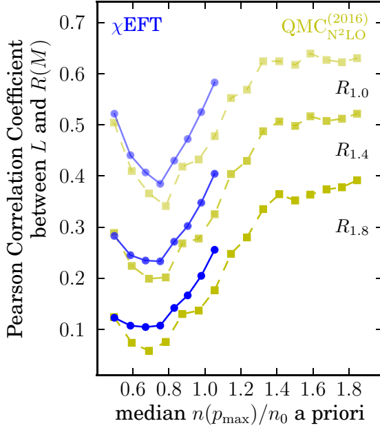
FIG. 11. Pearson correlation coefficients between L and R(M) for marginalized \chi EFT results (blue circles, solid lines) and \text{QMC}_{\text{N}^2\text{LO}}^{(2016)} (yellow squares, dashed lines). In order from lightest to darkest lines (top to bottom), we plot the correlation between L and R(1.0 M_\odot) , R(1.4 M_\odot) , and R(1.8 M_\odot) .
