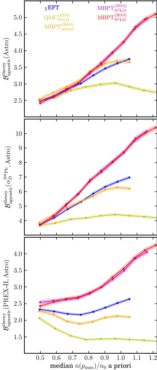
FIG. 6. Bayes factors between priors conditioned on \chi EFT calculations up to different p_{\max} vs the priors not conditioned on \chi EFT at all for (top) astrophysical data, (middle) Astro+ \alpha_D^{208\text{Pb}} , and (bottom) Astro+PREX-II data. We show results for the \chi EFT-marginalized calculations (blue) as well as the QMC _{\text{N}^2\text{LO}}^{(2016)} (yellow), MBPT _{\text{mixed}}^{(2010)} (orange), MBPT _{\text{N}^3\text{LO}}^{(2013)} (purple), and MBPT _{\text{N}^3\text{LO}}^{(2019)} (red) calculations separately.
