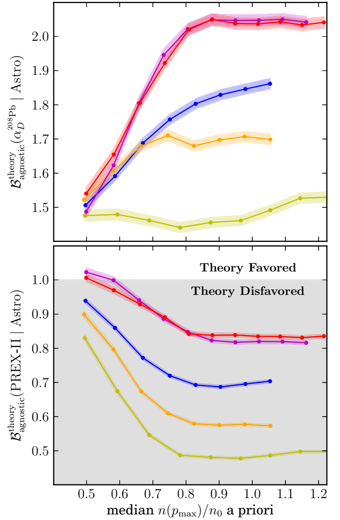
FIG. 7. Bayes factors between priors conditioned on \chi EFT vs priors not conditioned on \chi EFT at all for different nuclear data when we first condition on the astrophysical observations (include them as part of the prior). We show the results for (top) \alpha_D^{208\text{Pb}} and (bottom) PREX-II data.
