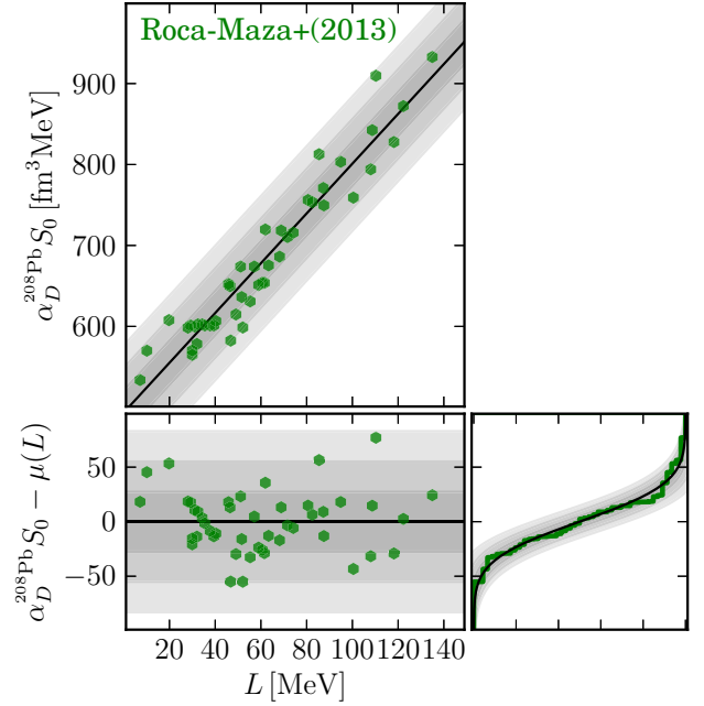
FIG. 2. Analogous to Fig. 1, but showing the conditional uncertainty for P(\alpha_D^{208\text{Pb}} S_0 | L) , modeled as a Gaussian with mean given by Eq. (25), based on Ref. [10]. Shaded bands represent 1\sigma , 2\sigma , and 3\sigma uncertainty within our model. We again obtain good quantitative agreement between our uncertainty model and the observed scatter of the theoretical models.
