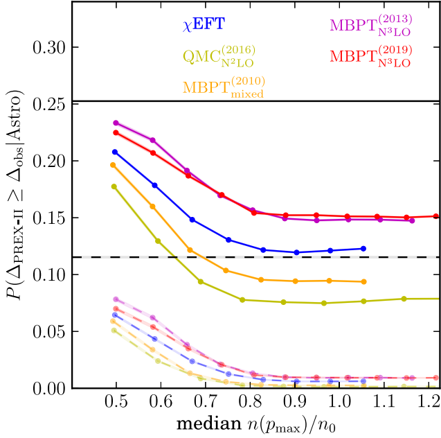
FIG. 5. Probability of PREX-II disagreeing with posteriors conditioned on \chi EFT up to p_{\max} by at least the measured difference given experimental uncertainties ( p values, solid lines ). We also show the p values for a hypothetical experiment producing the same mean as PREX-II with half the uncertainty ( dashed lines ). Results are given for nonparametric Astro-only posteriors ( black horizontal lines ), \chi EFT-marginalized ( blue ), \text{QMC}_{\text{N}^2\text{LO}}^{(2016)} ( yellow ), \text{MBPT}_{\text{mixed}}^{(2010)} ( orange ), \text{MBPT}_{\text{N}^3\text{LO}}^{(2013)} ( purple ), and \text{MBPT}_{\text{N}^3\text{LO}}^{(2019)} ( red ).
