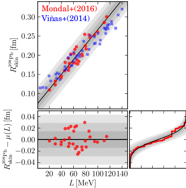
FIG. 1. Uncertainty relation between R_{\text{skin}}^{208\text{Pb}} and L modeled on the 31 models from Ref. [7] (red circles) compared with 47 models from Ref. [5] (blue squares). Left: We model the theoretical uncertainty with a conditional probability P(R_{\text{skin}}^{208\text{Pb}}|L) using a normal distribution with mean given by Eq. (24). Shaded bands correspond to 1\sigma , 2\sigma , and 3\sigma uncertainties for R_{\text{skin}}^{208\text{Pb}} at each L . Bottom right: Predicted cumulative distribution of residuals and empirical distribution based on the fit to Ref. [7], showing good quantitative agreement between our model and the scatter between the theoretical calculations. We note that the models from Ref. [5] are systematically shifted compared to Ref. [7], but they are well represented by our uncertainty model.
