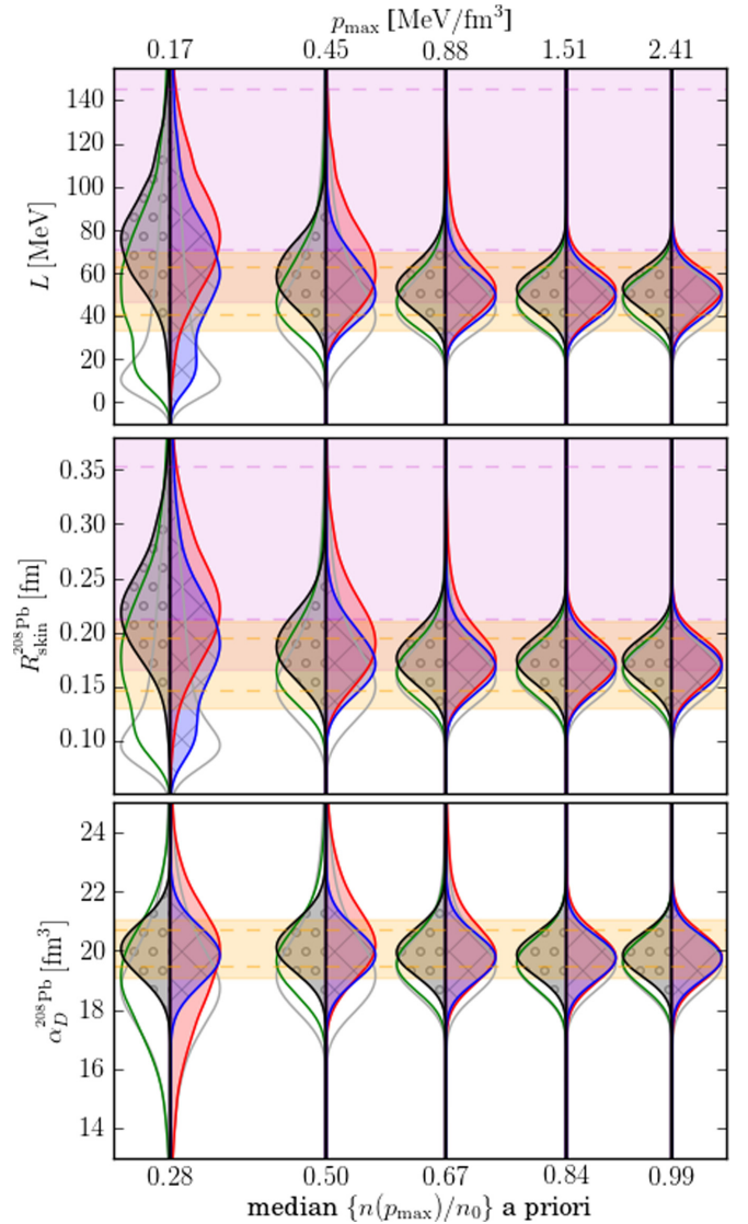
FIG. 4. Priors (grey, unshaded), Astro-only posteriors (left side of violins, green unshaded), Astro+PREX-II posteriors (right side of violins, red shaded), Astro+ \alpha_D^{208\text{Pb}} posteriors (right side of violins, blue shaded+hatched), and Astro+PREX-II+ \alpha_D^{208\text{Pb}} posteriors (left side of violins, grey shaded+dots) for \chi EFT-marginalized results as a function of the maximum pressure up to which we trust \chi EFT. The left-most curves (median n \sim 0.3n_0 ) are equivalent to the nonparametric results in Fig. 3. Horizontal bands (dashed lines) correspond to 90% ( 1\sigma ) credible regions from PREX-II [21] ( R_{\text{skin}}^{208\text{Pb}} , pink) and the electric dipole polarizability [8] ( \alpha_D^{208\text{Pb}} , orange). When translating experimental data to their correlated properties in this figure (e.g., horizontal \alpha_D^{208\text{Pb}} bands for L and R_{\text{skin}}^{208\text{Pb}} ), we employ our uncertainty relations in the theoretical correlations [Eqs. (24) and (25), assuming S_0 = 32.5 MeV for the latter].
