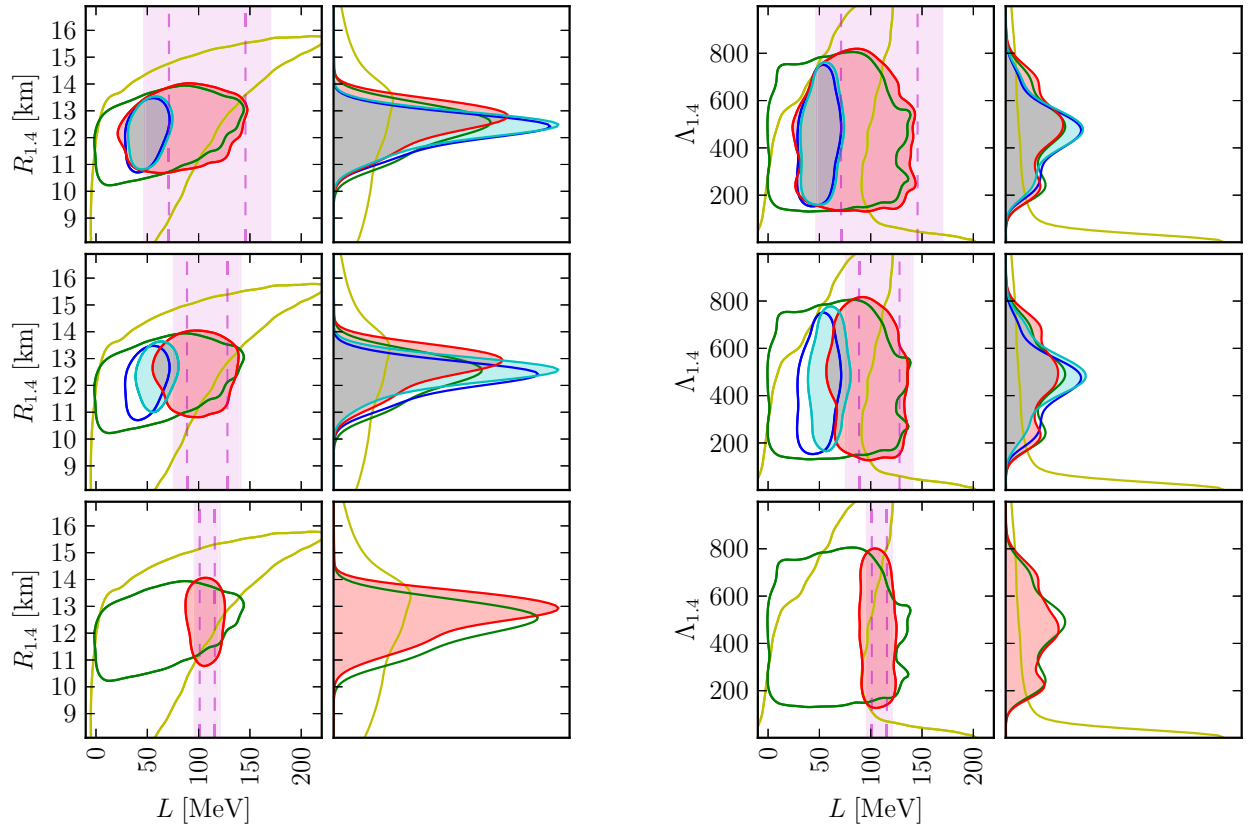
FIG. 12. Correlations between ( left ) R_{1,4} , ( right ) \Lambda_{1,4} and L when we model the PREX-II measurement with different uncertainties: the actual measurement uncertainty ( top ), a hypothetical measurement with half the PREX-II uncertainty ( middle ), and a hypothetical measurement with vanishingly small uncertainty for R_{\text{skin}}^{208\text{Pb}} ( bottom ). Colors and shading match those in Fig. 9. We see that even a perfect measurement of R_{\text{skin}}^{208\text{Pb}} does not significantly alter our knowledge of the macroscopic properties of typical astrophysical NSs within the nonparametric inference.
