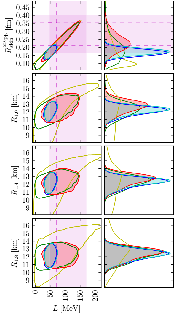
FIG. 10. Correlations of R_{\text{skin}}^{208\text{Pb}} and the radii of NSs with M = 1.0 M_\odot , 1.4 M_\odot , and 1.8 M_\odot with L . Colors and shading match those in Fig. 9.
