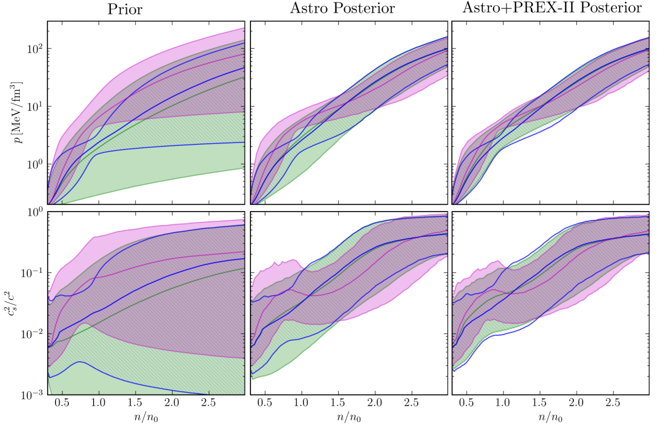
FIG. 8. Median and 90% symmetric credible regions for the prior ( left ), Astro-only posterior ( middle ), and Astro+PREX-II posterior ( right ) for all EOS and all values of L ( green ), EOS with 30 \text{ MeV} < L < 70 \text{ MeV} ( hatched blue ), and EOS with 100 \text{ MeV} < L ( purple ). The main effect of the PREX-II data is to rule out some of the very soft EOS at low densities ( L \lesssim 30 \text{ MeV} ).
