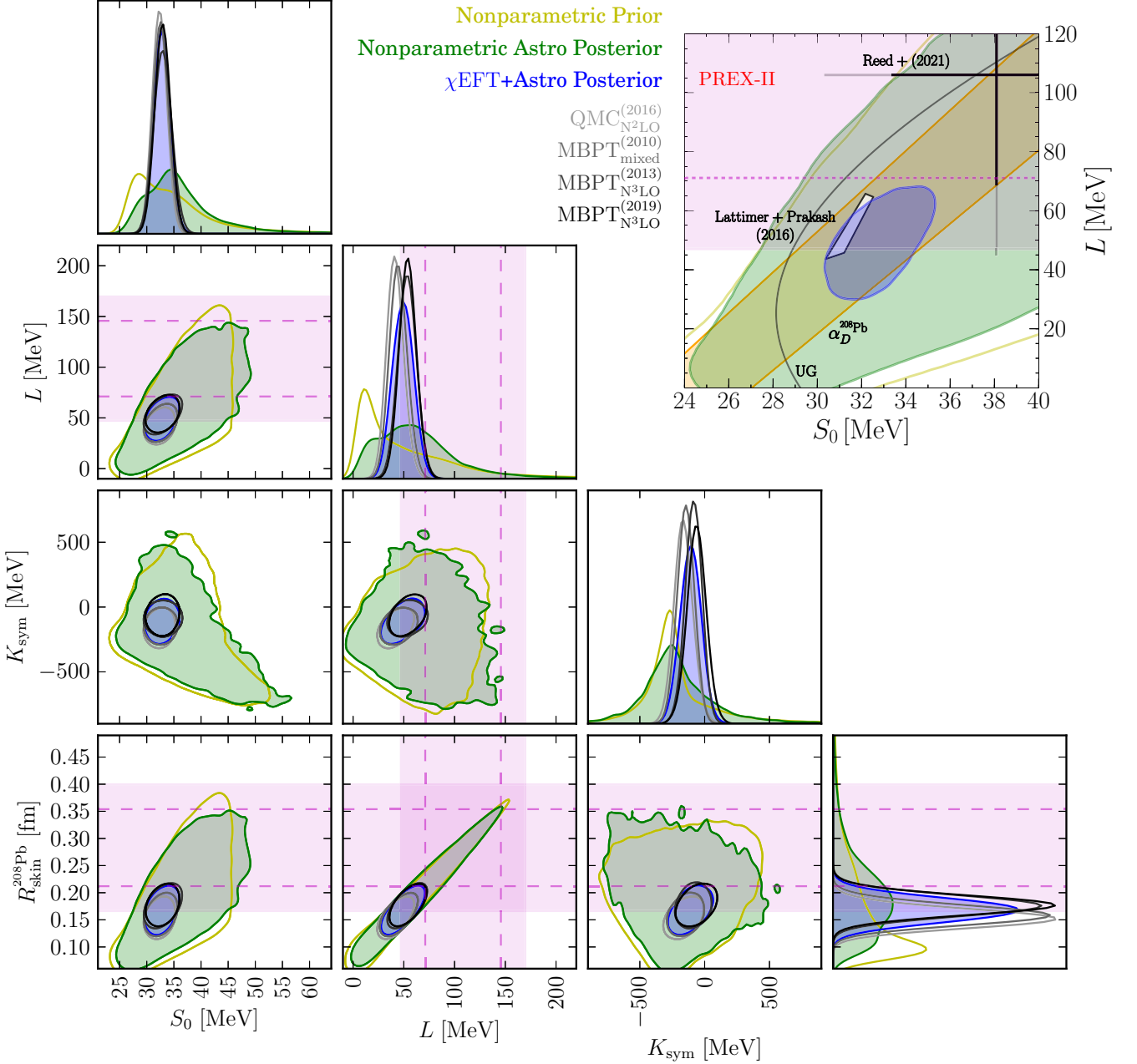
FIG. 3. Correlations between S_0 , L , K_{\text{sym}} , and R_{\text{skin}}^{208\text{Pb}} within our nonparametric prior (unshaded yellow) and Astro-only posterior (shaded green) as well as the \chi\text{EFT} -marginalized (shaded blue), \text{QMC}_{\text{N}^2\text{LO}}^{(2016)} , \text{MBPT}_{\text{mixed}}^{(2010)} , \text{MBPT}_{\text{N}^3\text{LO}}^{(2013)} , and \text{MBPT}_{\text{N}^3\text{LO}}^{(2019)} Astro-only posteriors (unshaded greys, ordered from lighter to darker with increasing L ; see Table I). Joint distributions show 90% credible regions, and the horizontal bands (pink) represent PREX-II 90% credible regions and dashed lines the corresponding 68% ( 1\sigma ) regions. The expanded ( S_0 , L ) panel (upper right) compares our nonparametric prior, Astro-only posterior, and \chi\text{EFT} +Astro posterior to other constraints: (white region) Lattimer and Prakash [69] (overlap region of various nuclear experimental constraints), the unitary-gas (UG) bound from Ref. [70], and the values reported by Reed et al. [22] based on the PREX-II results. In addition, we show the correlation obtained from the experimental \alpha_D^{208\text{Pb}} [8] using Eq. (25).
