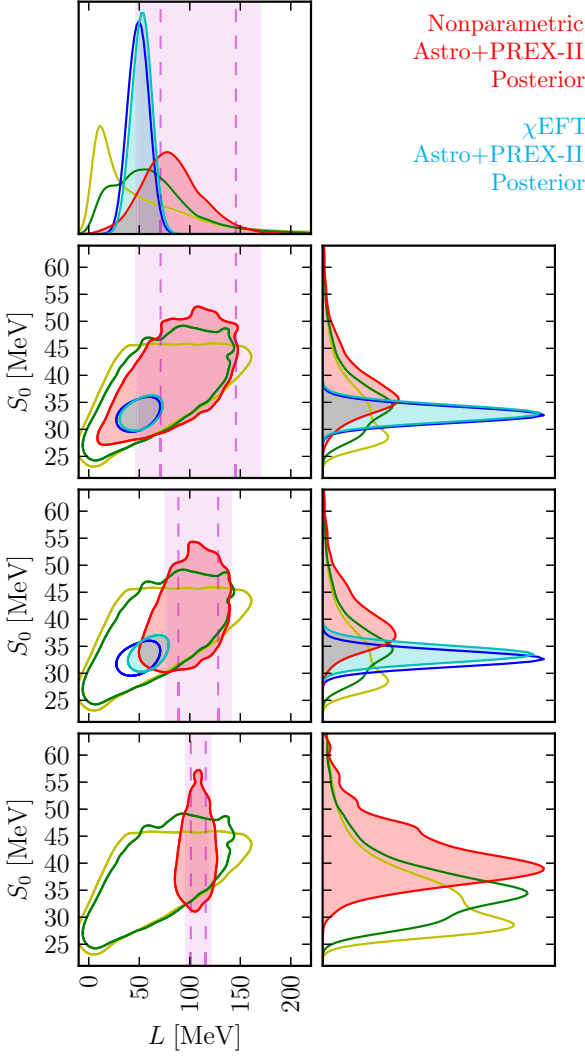
FIG. 9. Correlations between S_0 and L when we model the PREX-II estimate with different uncertainties: ( top ) the actual measurement uncertainty, ( middle ) a hypothetical measurement with half the PREX-II uncertainty, and ( bottom ) a hypothetical measurement with vanishingly small uncertainty for R_{\text{skin}}^{208\text{Pb}} . We show the nonparametric prior ( unshaded yellow ), Astro-only posterior ( unshaded green ), and Astro+PREX-II posterior ( shaded red ) as well as the \chi EFT-marginalized Astro-only posterior ( unshaded blue ) and Astro+PREX-II posterior ( shaded light blue ). As in Fig. 3, ( pink ) shaded vertical bands represent (real and hypothetical) PREX-II 90% credible regions and dashed lines show the 1\sigma credible regions uncertainty. Improved measurements of R_{\text{skin}}^{208\text{Pb}} are still consistent with a wide range of S_0 within the nonparametric inference.
