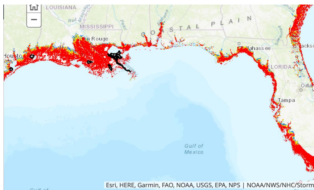
Figure 1. National Hurricane Center prediction of the “maximum of maximum envelope water” (MOMs) caused by storm surges associated with landfalling category five hurricane over the central and eastern regions of the Gulf Coast. The red areas could expect inundation to exceed 9 feet (~3m) above existing ground levels. Levees currently protect areas shown in black. This public domain image from NOAA was also presented in [31,86].
