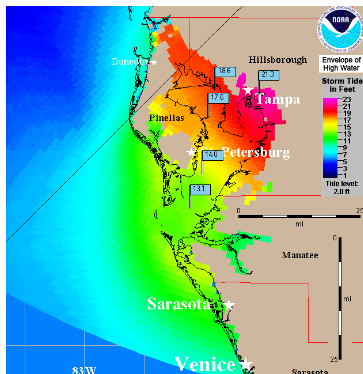
Figure 2. Predicted storm tide (storm surge superimposed on high tide) height for a category 4 hurricane making land fall on Tampa Bay at high tide. Due to the funneling effects of the bay, areas in the upper (northeastern) part of the bay where Tampa's city center is located could expect over 20 feet of flooding. Model results from NOAA's National Hurricane Center utilizing the sea, lake, and overland surges from hurricanes (SLOSH) model. Source: Public domain NOAA image also presented in [87].
