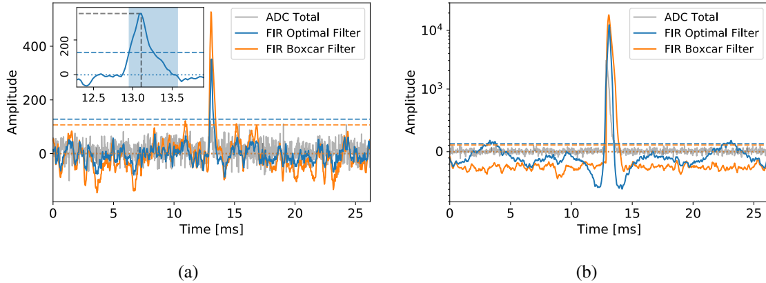
Figure 5. ADC readout traces and two simulated FIR outputs from an injected AWG pulse with an amplitude of 3\ \sigma_n (a) and 100\ \sigma_n (b) where the FIRs are configured as an optimal filter and a boxcar filter. The dashed and dotted lines mark the activation and deactivation thresholds. The blue shaded area in the inset of (a) marks the peak search window defined by the FIR filtered traces crossing above and falling below the activation and deactivation thresholds. The gray dashed lines indicate the final trigger peak amplitude and time stamp. The filtered trace of the optimal filter in (b) going above the activation threshold demonstrates the occurrence of echo triggers close to large pulses, the filtered trace of the boxcar filter does not show the same effect.
